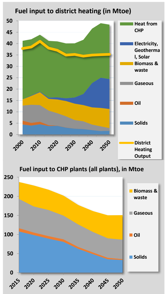
FIGURE 42: FUEL INPUT FOR STEAM GENERATION
