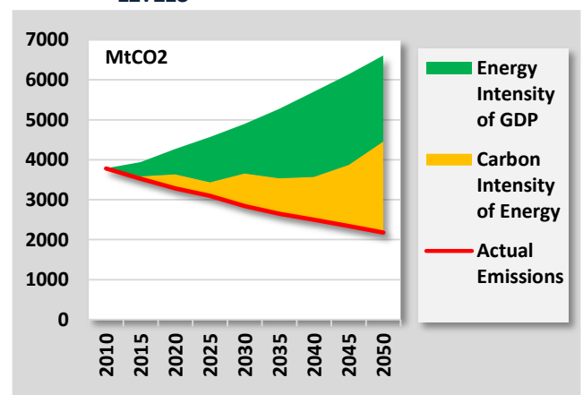
FIGURE 52: DECOMPOSITION OF ENERGY-RELATED CO 2 EMISSION REDUCTION RELATIVE TO PROJECTION WITH CO 2 INTENSITY OF GDP FROZEN TO 2010 LEVELS
