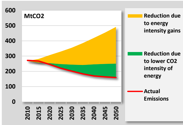
FIGURE 57: DECOMPOSITION OF ENERGY-RELATED CO 2 EMISSION REDUCTION IN THE TERTIARY SECTOR RELATIVE TO PROJECTION WITH CO 2 INTENSITY OF ACTIVITY FROZEN TO 2010 LEVELS
