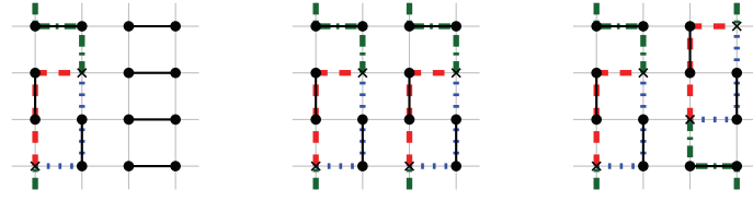
Fig. 12. Toroidal grid T_{4,4} with the three possible sets of unsaturated vertices, corresponding maximal matchings, and augmenting path forests, for Lemma 22.
