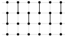
Fig. 7. Matching M in Y_{6,4} for Lemma 16.
