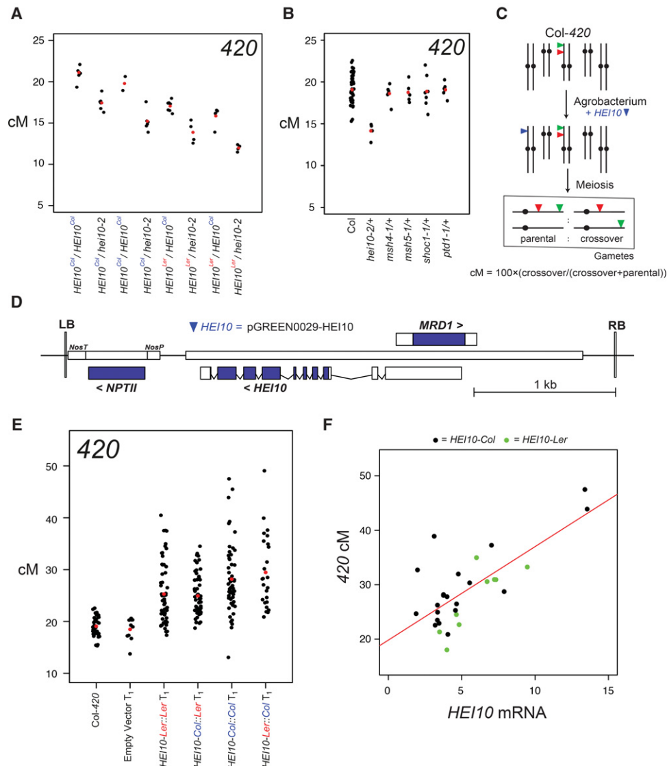
Figure 4. HEI10 is a dosage-sensitive regulator of Arabidopsis crossovers. (A) 420 crossovers (in centimorgans) in F_1 individuals derived from crosses between HEI10^{Col} or HEI10^{Ler} homozygotes and wild-type (Col) or null hei10-2 mutants. Replicate individuals are shown as black dots, and mean values are shown as red dots. (B) 420 crossovers (in centimorgans) in F_1 individuals derived from crosses with interfering crossover ZMM pathway mutants. (C) Schematic showing the transformation of Col-420 with additional HEI10 copies (blue triangles). (D) Diagram illustrating the HEI10 T-DNA construct used for Arabidopsis transformation via Agrobacterium . (LB) T-DNA left border sequence; (RB) T-DNA right border sequences. (E) 420 crossover frequency (in centimorgans) in empty vector, HEI10^{Ler::Ler} , HEI10^{Col::Ler} , HEI10^{Ler::Col} , and HEI10^{Col::Col} transformants compared with untransformed Col-420/Col controls. Data from individual plants are shown as black dots, and mean values are shown in red. (F) Correlation between 420 crossovers (in centimorgans) and HEI10 transcript levels measured by qRT-PCR from HEI10^{Col} (black) and HEI10^{Ler} (green) transformant flowers. A regression line is plotted in red.
