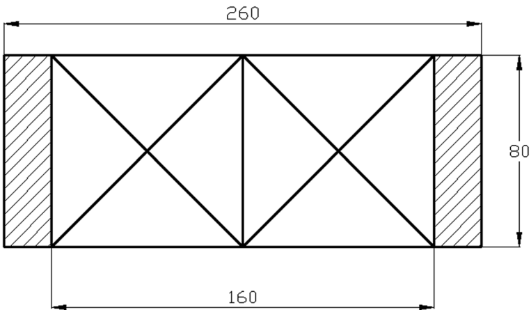
Fig. 2 Specimen's shape for bias extension test
