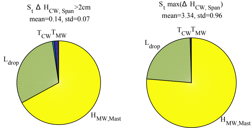
Figure 7: Sobol total indices for \Delta H_{CW,Span} > 2cm (left) and max(\Delta^2 H_{CW,Span}) (right)
