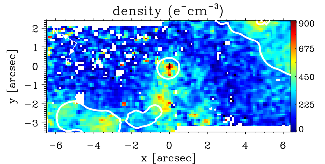
Figure 6. Electron density map derived from the flux ratio [SII]\lambda\lambda 6716/6731 assuming a temperature T = 10^4 \text{ K} . The solid white contours mark the most prominent features visible in the H\alpha flux map.
