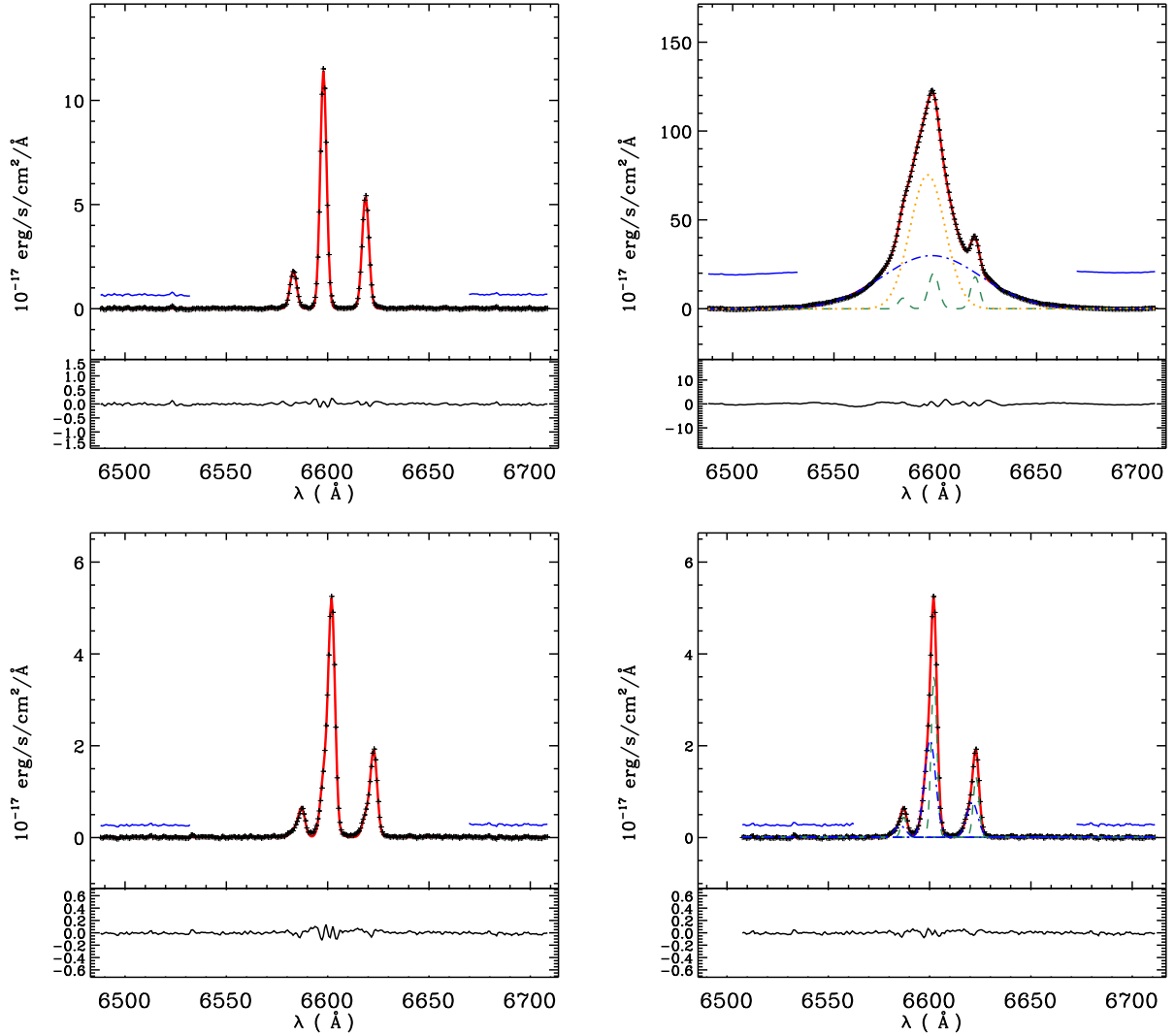
Figure 2. Fit of the [NII] \lambda\lambda 6548,6583 and H \alpha emission lines. Top left: example of single Gaussian fit. The horizontal blue lines mark the continuum level before it was subtracted. Top right: fit at the nucleus. Two Gaussians were used to model the broad H \alpha (blue dot-dashed and orange short-dashed). The green long-dashed Gaussians represent the underlying narrow components. Bottom left: example of a fit with Gauss-Hermite polynomials. Bottom right: same spectrum shown in the previous panel, but in this case modelled with two Gaussians to extract the velocity of the component associated with the asymmetry (blue dot-dashed Gaussian).
