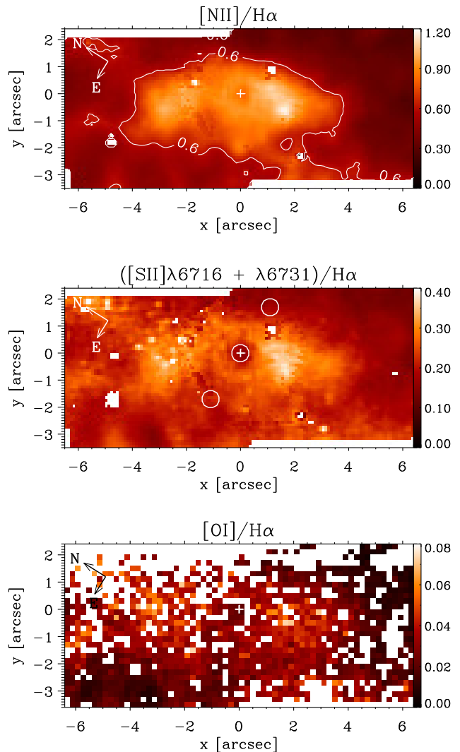
Figure 7. Flux ratios [NII] \lambda 6583/ H\alpha , [SII] (\lambda 6716 + \lambda 6731)/ H\alpha and [OI] \lambda 6300/ H\alpha . Spaxels where the relative error on the ratio is equal to or larger than 50% have been masked out (blank pixels). A contour corresponding to [NII]/ H\alpha = 0.6 is plotted in the top panel; [NII]/ H\alpha > 0.6 ( \log 0.6 = -0.2 ) is characteristic of AGN photoionization. Solid circles in the central panel highlight the regions used to extract the data plotted in the BPT diagrams.
