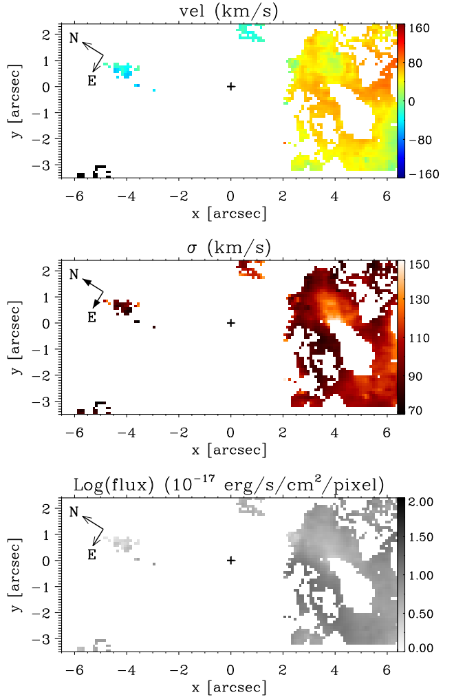
Figure 5. Maps derived by fitting two Gaussians to the [NII]\lambda 6583 emission lines characterized by a skewness |h_3| \geq 0.05 . Maps shown here represent the asymmetric component. Top : velocity. Center : velocity dispersion. Bottom : flux. The velocity map is shown after subtracting a systemic velocity of 1671 \text{ km s}^{-1} .
