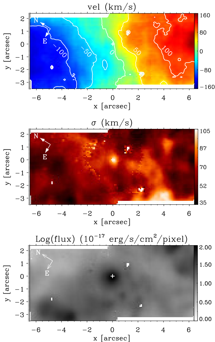
Figure 3. Maps derived by fitting a Gaussian profile to the narrow component of the [NII] emission line. Top: velocity. Center: velocity dispersion. Bottom: flux. The velocity map is shown after subtracting a systemic velocity of 1671 \text{ km s}^{-1} (derived from the modeling described in §5.1). The cross at (0,0) marks the continuum brightness peak.
