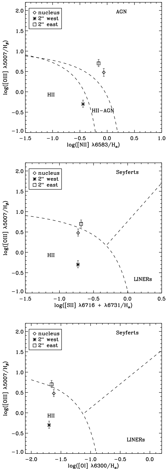
Figure 8. BPT diagrams for line ratios computed over circular regions of 0''.3 in radius centered at the nucleus, and 2'' east and west of the nucleus as indicated in the middle panel of Fig.7. Values for the [\text{OIII}]/\text{H}\beta ratio have been taken from Schulz et al. (1999). Horizontal error bars are approximately of the same size of the symbols. The dashed boundary lines are taken from Kewley et al. (2006).
