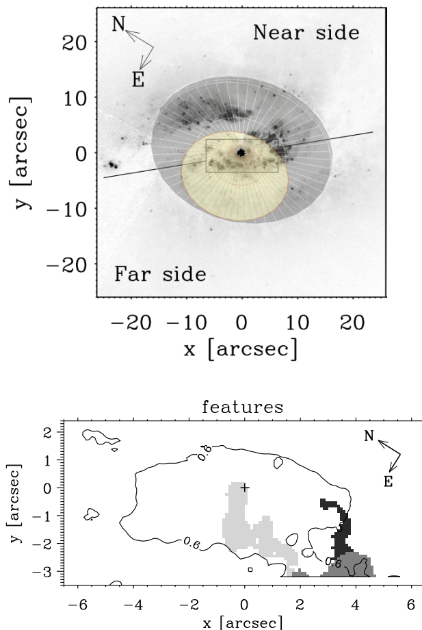
Figure 10. Top: as in Fig.1, with a cartoon representing the plane of the galaxy (large grey disk) and the approaching AGN radiation cone (in yellow, cartoon made with the Shape software, Steffen et al. 2011). Bottom: map of the observed features suggestive of outflowing gas: fan-shaped blueshifted velocity excess coincident with enhanced electron density (light gray), clear evidence for a second spectral component, suggestive of unresolved split lines (dark grey), flat-topped line profiles suggestive of unresolved split lines (black and dark grey). The solid line corresponds to [\text{NII}]/\text{H}\alpha = 0.6 , as in Fig.7. Points inside the contour are characterized by [\text{NII}]/\text{H}\alpha \geq 0.6 , suggestive of AGN photoionization.
