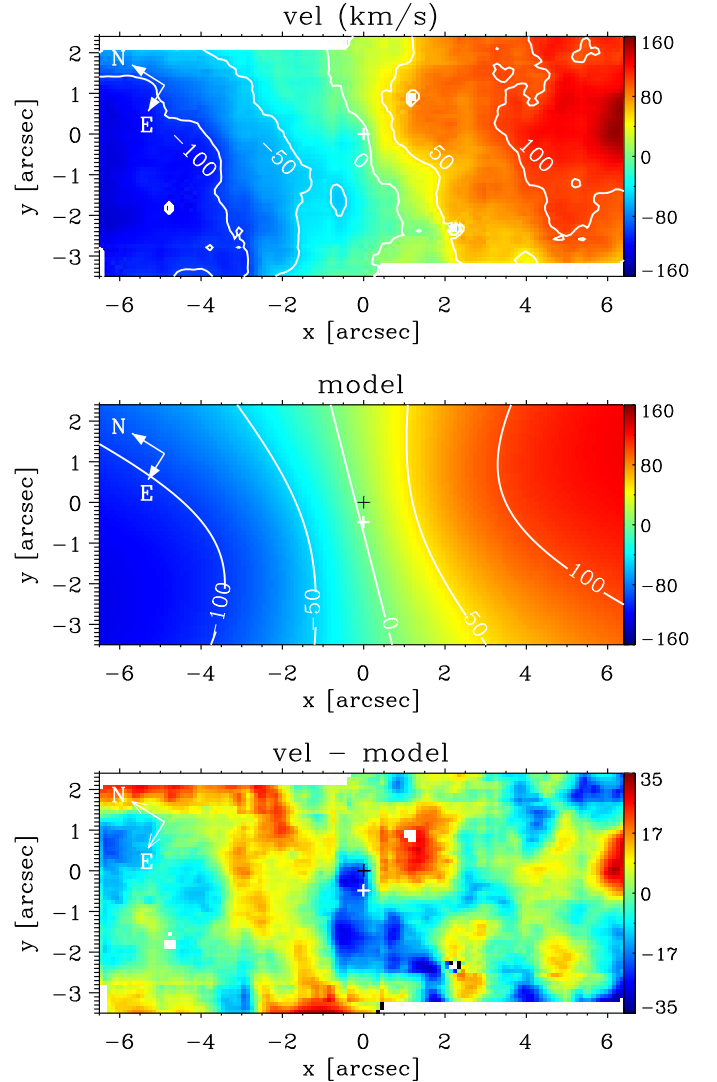
Figure 9. Maps derived from the fit to the narrow component of the [NII] emission line. Top : observed velocity field. Center : model. Bottom : residual. The velocity map is shown after subtracting a systemic velocity of 1671 km s -1 , derived from the fit. The black cross at (0,0) marks the continuum brightness peak. The white cross marks the kinematical center derived from the fit.
