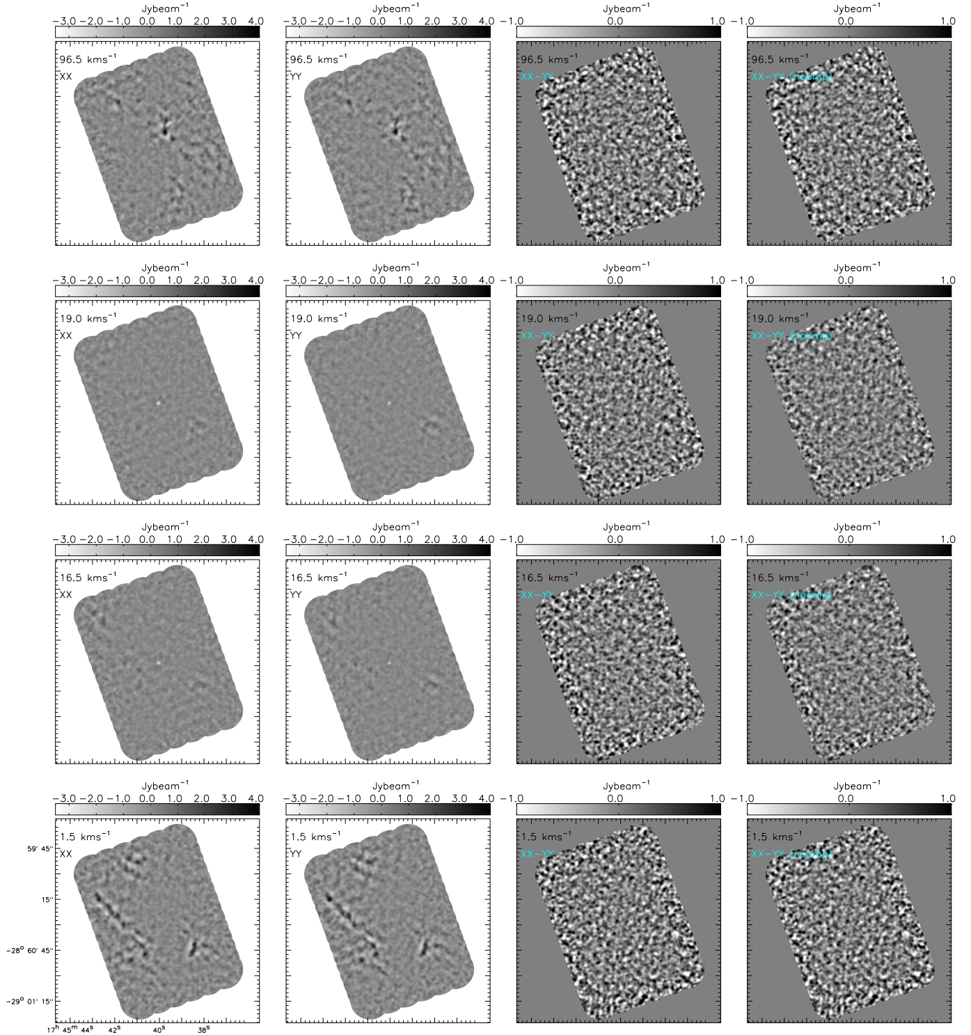
Fig. 7. Left to right columns: XX , YY , XX - YY , and XX - a^{\text{CI}}(v)YY synthesized intensity maps of selected velocity channels. These images were generated using the 12 m array data only (Sect. 2), and were further tapered by a Gaussian weighting function of \text{FWHM} = 1''.5 . The CI line emission close to v_{\text{lsr}} \sim 20 \text{ km s}^{-1} is subject to foreground absorption, such that the images are dominated by the point-like absorption signature against Sgr A*. Extended CI emission features surrounding Sgr A* are present away from v_{\text{lsr}} \sim 20 \text{ km s}^{-1} .
