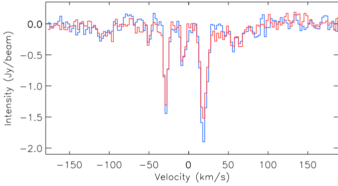
Fig. 8. Line spectra of Cl taken from a single synthesized beam area surrounding Sgr A*. The blue and red lines present the XX and YY polarizations.
