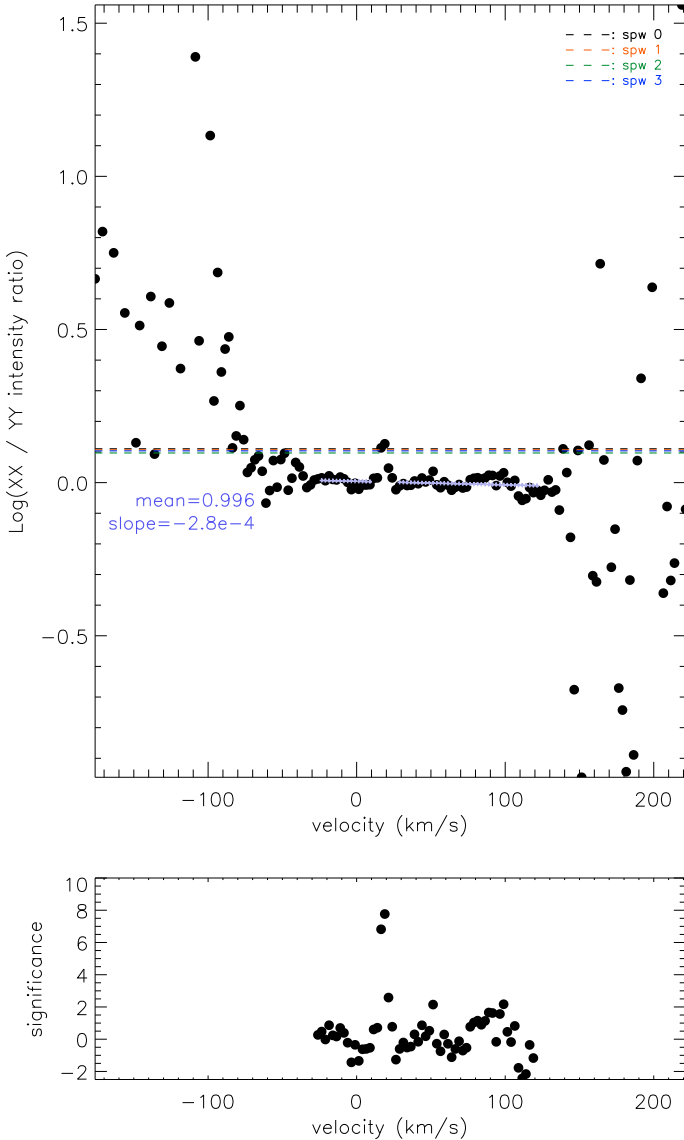
Fig. 6. Top panel: derived intensity ratio between the XX and the YY correlations ( F_{XX}^{\text{Cl}}(\nu)/F_{YY}^{\text{Cl}}(\nu) ) from the Cl line velocity channel synthesized image, as a function of v_{\text{lsr}} . We overplotted the XX and YY intensity ratios derived from the continuum data of the inner 7 12 m array mosaic fields (dashed lines, color coding the four spectral windows). The large scattering in the redshifted and blueshifted ends are because we did not detect Cl emission or absorption in those channels, and therefore fittings of F_{XX}^{\text{Cl}}(\nu)/F_{YY}^{\text{Cl}}(\nu) did not converge. We performed linear regression for the high S/N spectral channels, and derived the \pm 1 standard deviation ( \sigma_v^{\text{Cl}} ) of the differences from the regression line. The result of the linear regression is shown by light blue symbols. We plot (F_{XX}^{\text{Cl}}(\nu)/F_{YY}^{\text{Cl}}(\nu))/(\sigma_v^{\text{Cl}}) in the bottom panel .
