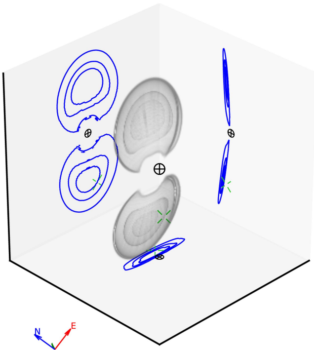
Figure 1. Volume rendering of the 20%, 50%, and 90% credible levels of a typical two-detector early Advanced LIGO event. The three planes are perpendicular to the principal components of the probability distribution. The observer’s position (the Earth) is at the origin. The green reticle shows the true position of the source. The compass in the bottom left corner shows the basis vectors of the equatorial coordinate system.
