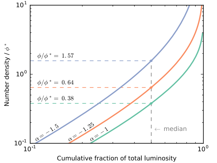
Figure 3. Tradeoff between completeness and the number of galaxies, assuming various Schechter luminosity functions. The horizontal axis is the cumulative fraction of the total luminosity in the local universe. The vertical axis is the number density of galaxies in units of \phi^* .
