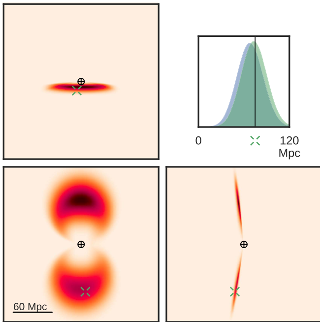
Figure 2. Left panel: marginal posterior probability distribution in the principal planes, as in Figure 1. The inset shows the marginal distance posterior distribution integrated over the whole sky (blue) and the conditional distance posterior distribution in the true direction of the source (green). Right panel: volume rendering of the 90% credible region superimposed over a slice of the galaxy group map of Tully (2015). The most massive galaxies inside the credible region are highlighted.
