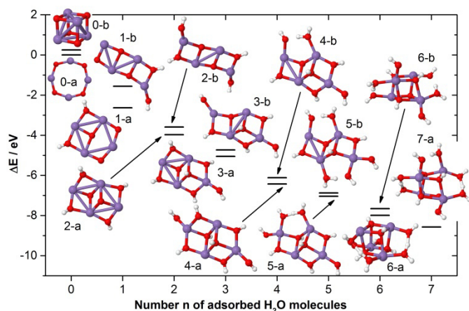
Fig 4 Calculated binding energies of n water molecules to \text{Mn}_4\text{O}_4^+ for the two lowest (except for \text{Mn}_4\text{O}_4(\text{H}_2\text{O})_7^+ ) energy isomers (denoted as energy difference \Delta E with respect to the bare ring-like \text{Mn}_4\text{O}_4^+ cluster), plotted along with the corresponding structures. 8 Mn, O, and H atoms are depicted as purple, red, and white spheres, respectively.
