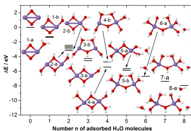
Fig. 6 Calculated binding energies of n water molecules to \text{Mn}_2\text{O}_2^+ for different isomeric structures (denoted as energy difference \Delta E with respect to the bare rhombic \text{Mn}_2\text{O}_2^+ cluster, shown at the top left corner), plotted along with the corresponding structures. Mn, O, and H atoms are depicted as purple, red, and white spheres, respectively.
