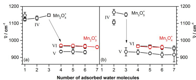
Fig 8 Experimentally obtained band centers of signals observed in two characteristic spectral regions as a function of the number of adsorbed water molecules. (a) Signals for the di-manganese oxide clusters \text{Mn}_2\text{O}_3(\text{H}_2\text{O})_n^+ ( n = 4 - 7 ) (shown as red circles) and \text{Mn}_2\text{O}_4(\text{H}_2\text{O})_n^+ ( n = 1 - 6 ) (black squares). (b) Signals for the tri-manganese oxide clusters \text{Mn}_3\text{O}_4(\text{H}_2\text{O})_n^+ ( n = 4 - 6 ) (red circles) and \text{Mn}_3\text{O}_5(\text{H}_2\text{O})_n^+ ( n = 2 - 7 ) (black squares). The error bars represent the FWHM. The lines are drawn to guide the eye. The labels IV, V, and VI refer to the signals in Figure 7.
