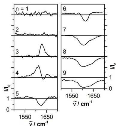
Fig. 2 Measured IR-MPD spectra of the complexes \text{Mn}_2\text{O}_2(\text{H}_2\text{O})_n^+ ( n = 1 - 9 ) in the spectral region of 1500 - 1700 \text{ cm}^{-1} which is characteristic for the HOH bending mode of intact water molecules. Plotted is the mass signal intensity ratio I/I_0 with ( I ) and without ( I_0 ) laser light, as a function of the incident laser wavenumber \tilde{\nu} .
