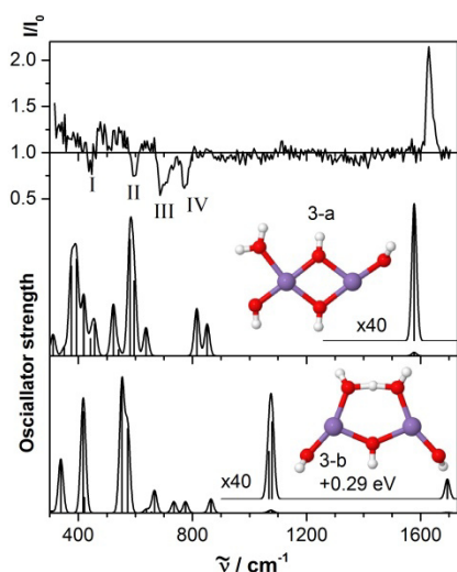
Fig. 5 IR-MPD spectrum (top panel) and calculated vibrational spectra of the two lowest energy isomeric structures of \text{Mn}_2\text{O}_2(\text{H}_2\text{O})_3^+ ; the ground-state (marked as 3-a) and the first higher-in-energy isomer (3-b). The calculated spectra (sticks) are convoluted with a Gaussian line shape function with a FWHM of 20\text{ cm}^{-1} . In the structural models, Mn, O, and H atoms are depicted as purple, red, and white spheres, respectively.
