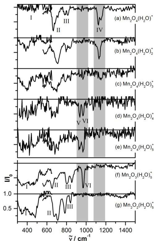
Fig. 7 IR-MPD spectra of (a)–(e) the cluster complexes \text{Mn}_2\text{O}_4(\text{H}_2\text{O})_n^+ ( n = 1 - 5 ) with two oxygen atoms in excess, (f) the cluster complex \text{Mn}_2\text{O}_3(\text{H}_2\text{O})_5^+ with one oxygen atom in excess, as well as (g) the stoichiometric \text{Mn}_2\text{O}_2(\text{H}_2\text{O})_5^+ cluster, in the spectral region of 300–1500 \text{cm}^{-1} . Plotted is the mass signal intensity ratio I/I_0 with (I) and without ( I_0 ) laser light as a function of the laser wavenumber \tilde{\nu} .
