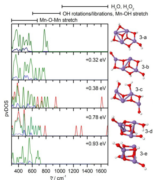
Fig. 1 Projected vibrational density of states (pvDOS, per \text{cm}^{-1} ) for five different isomeric structures of \text{Mn}_4\text{O}_4(\text{H}_2\text{O})_3^+ . The red curves represent the total vDOS whereas the green curve characterizes vibrational displacements of Mn atoms, the O atoms, and OH groups. The blue curve is the projection on the Mn atoms. For isomers 3-a (the ground state) and 3-b the red and green curves overlap in the whole frequency range obscuring the red curve. In the structural models, Mn, O, and H atoms are depicted as purple, red, and white spheres, respectively.
