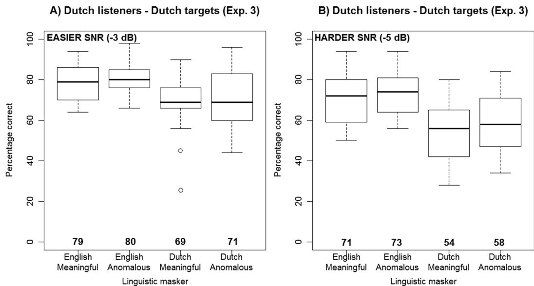
FIG. 4. Boxplots showing the interquartile ranges of intelligibility scores (in % correct) for Dutch listeners on Dutch target sentence recognition in (a) the easier SNR condition and in (b) the harder SNR condition (Experiment 3). Whiskers extend to the most extreme data point that is no more than 1.5 times the interquartile range of the box. The mean is given at the bottom of each plot.
