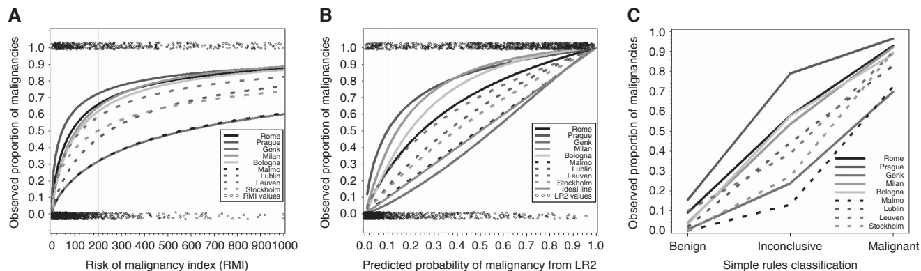
Figure 2. Centre-specific calibration curves (Cox logistic recalibration) for RMI ( A ), LR2 ( B ), and proportions for SRs ( C ). Vertical lines crossing the x axis for RMI (200) and LR2 (0.1, i.e., 10% risk) represent the original cutoff to define malignant disease. Scatter plots above and below the calibration curves for RMI and LR2 represent the distribution of predicted risks for LR2 and values for RMI for benign and malignant tumours, respectively. The x axis for RMI is limited to 1000. Oncology centres were: Rome, Prague, Milan, Leuven, Stockholm, Bologna and Lublin. Non-oncology centres were: Malmö and Genk.
