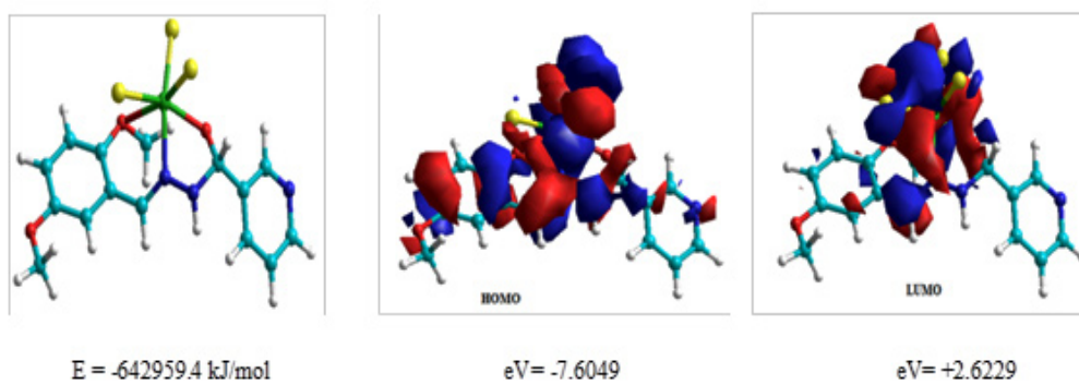
b. [\text{Mo}(\text{HL})\text{Cl}_3]
