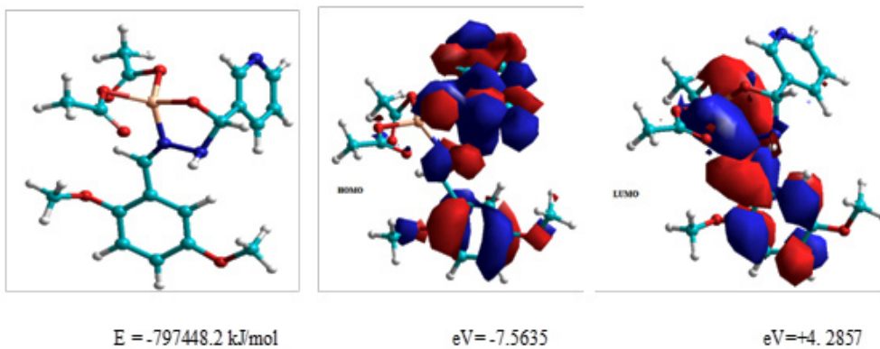
a. [\text{Mn}(\text{HL})(\text{CH}_3\text{COO})_2]
