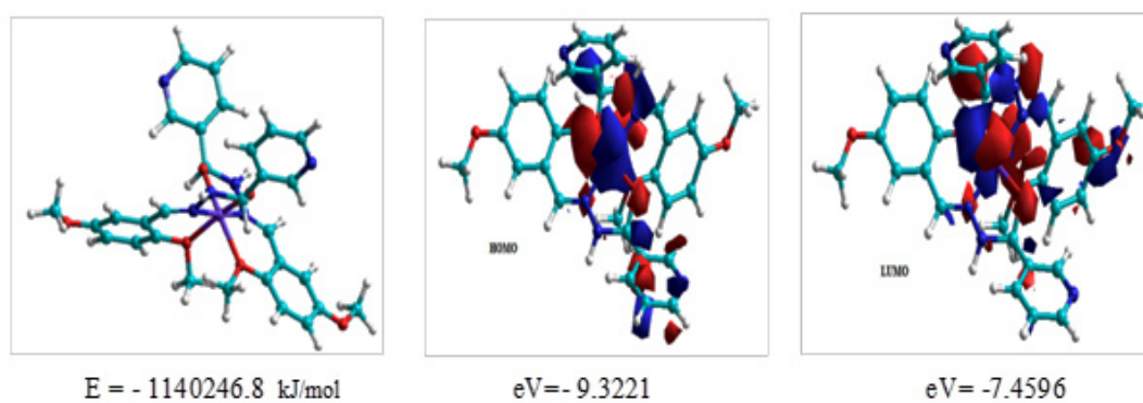
c. [\text{Cu}(\text{HL})_2]
