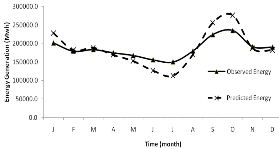
Figure-8. Model fitting for energy generation of Jebba hydropower dam.
