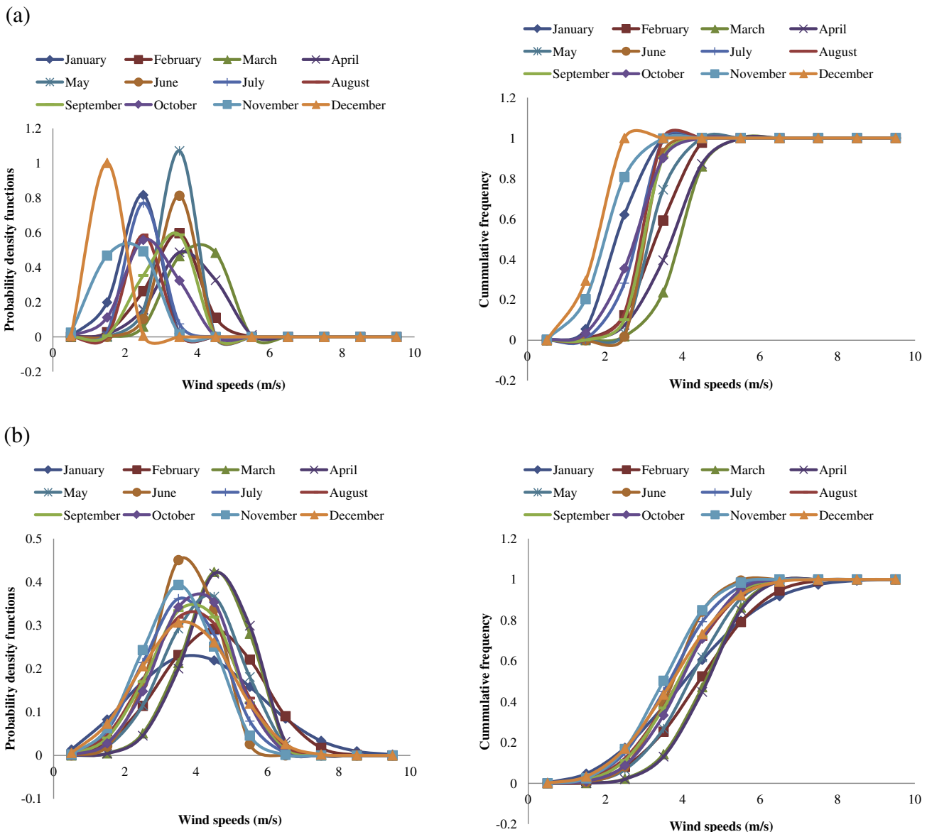
Fig. 3. Monthly wind speed probability density and cumulative distribution functions for (a) Ikrom (b) Ogoja (c) Calabar (d) Port Harcourt (e) Warri (f) Benin and (g) Asaba for the whole year.
