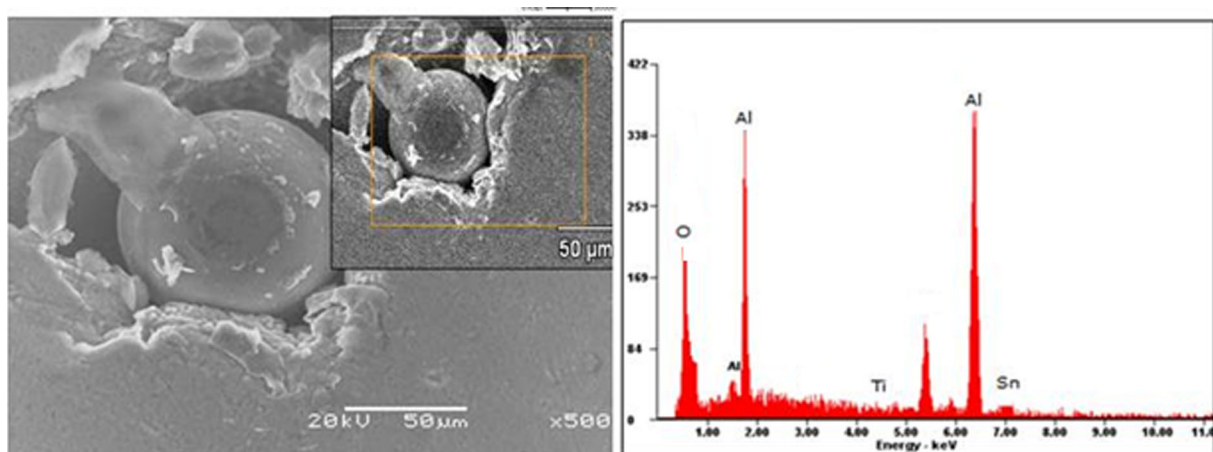
Fig. 3 SEM/EDS morphology of 10 wt.% TiO 2 /SnO 2 -inoculated A500 aluminum series
