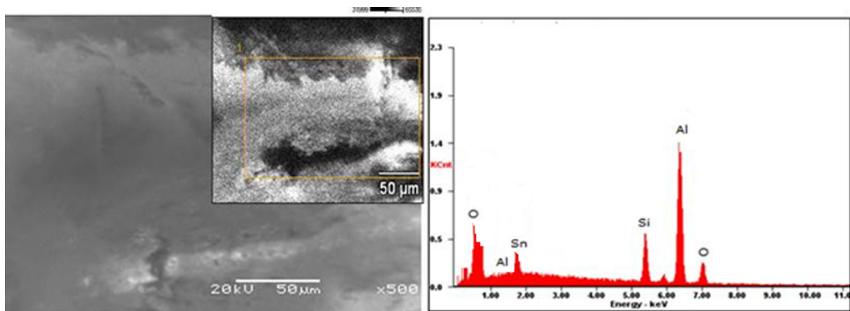
Fig. 2 SEM/EDS morphology of 5% SnO 2 -inoculated A500 aluminum series
