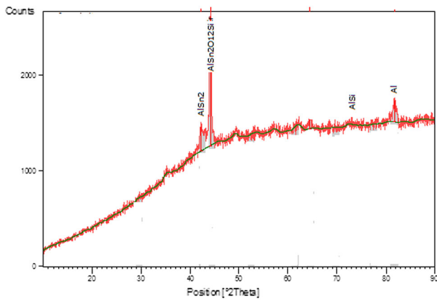
Fig. 4 XRD pattern of 5% SnO 2 -inoculated A500-Al-Si
