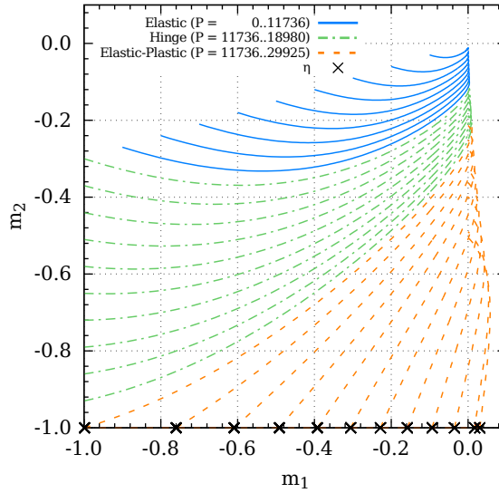
Figure 3.3: Stress profile.
