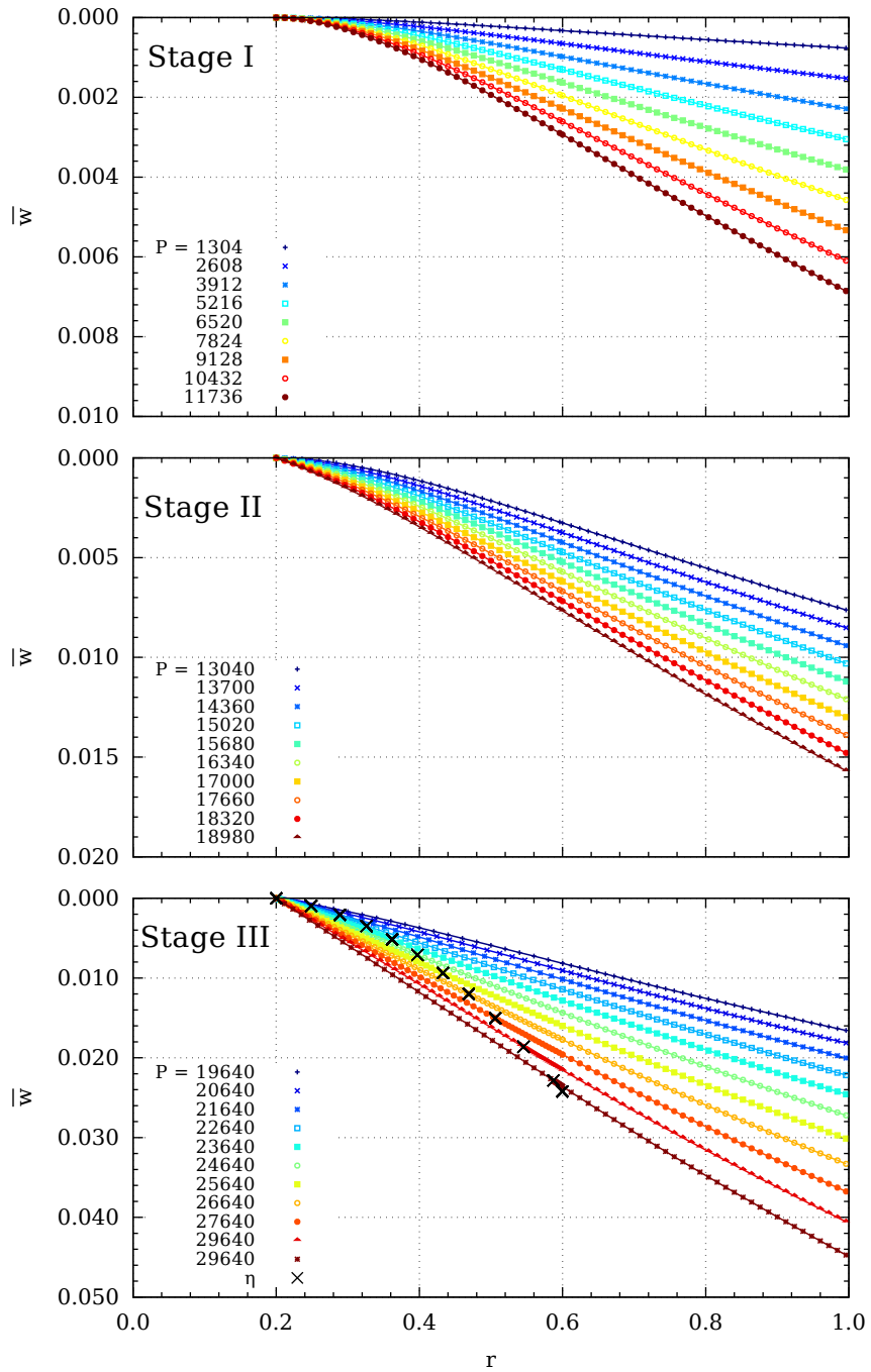
Figure 3.6: Deflections \bar{w} .
