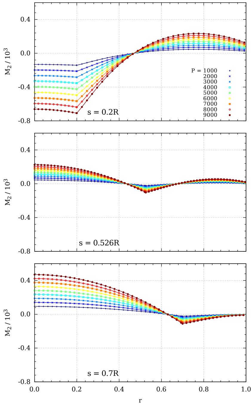
Figure 4.4: Circumferential moments.
