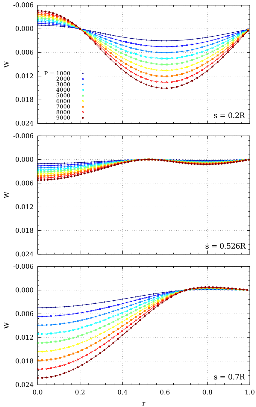
Figure 4.2: Deflections.
