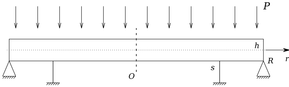
Figure 4.1: Circular plate with an additional support.
