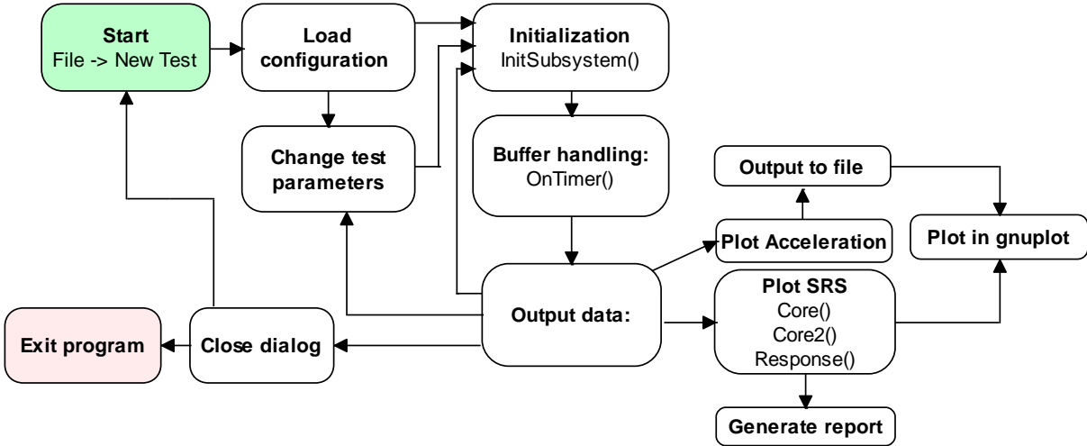
Figure 5.1: Software flowchart
