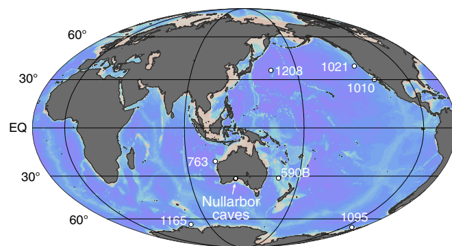
Fig. 2. Locality map showing Nullarbor caves in southern Australia and sites mentioned in the text. The map was produced using Ocean Data View (odv.awi.de).
