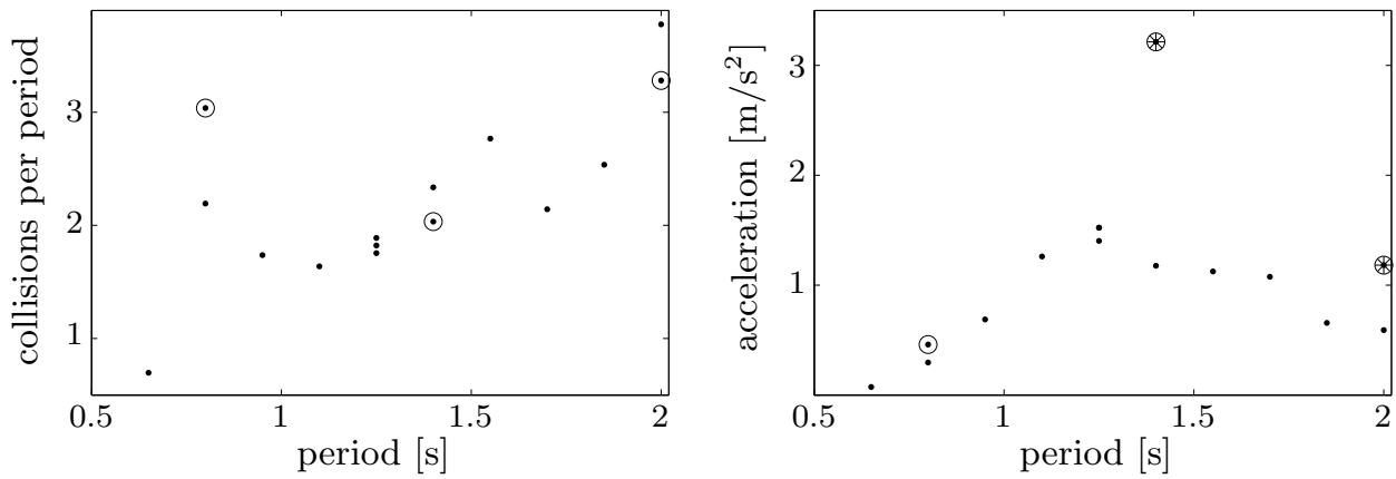
Figure 10: Mean number of collisions experienced by disks with accelerometers in middle row of high-concentration array per target wave period (left-hand panel), and corresponding mean magnitude of accelerations (right). Asterisks denotes tests in which one or more collisions saturates the signal.
