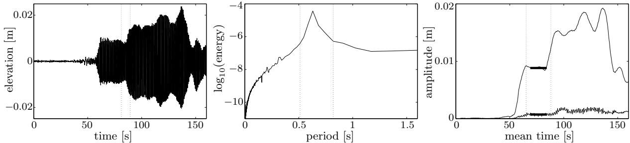
Figure 3: Example conversion of time series to representative amplitude in steady-state interval. Left-hand panel shows raw-surface-elevation time series from probe closest to wave maker, for test with target wave period 0.65 s and high-concentration array. Dotted vertical lines indicate a time window. Middle panel shows the energy spectrum for the indicated window. Dotted vertical lines indicate bins used to calculate the amplitude at the target period. Right-hand panel shows the amplitude at the target period and half the target period (smaller) as functions of mean time. Dotted vertical lines indicate the steady-state interval. Bars indicate the extracted amplitude and chosen interval.
