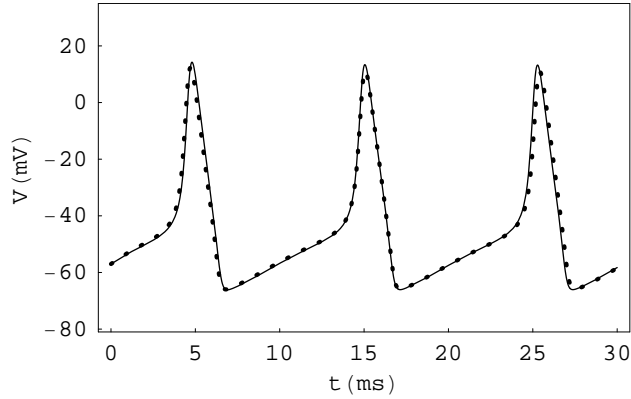
Figure 15: During a limit cycle solution of Eqs. (55) - (57), the two-stage activation of K^+ channels, defined by Eqs. (50) - (51) and \beta \gg \delta , \alpha \gg \gamma (solid line), may be approximated by a rate equation, Eqs. (14), (17), and (18) (dotted line). The rate functions \alpha(V) = 6.4 \exp[0.3(V - V_0)/25] , \beta(V) = 17.6 \exp[-1.4(V - V_0)/25] , \gamma(V) = 0.24 \exp[0.345(V - V_0)/25] , \delta(V) = 0.125 \exp[-0.312(V - V_0)/25] , \alpha_m(V) and \beta_m(V) defined by Eq. (52), V_m = 60 , \bar{g}_K = 36 mS/cm 2 , \bar{g}_{Na} = 120 mS/cm 2 , \bar{g}_L = 0.3 mS/cm 2 , V_K = -72 mV, V_{Na} = 55 mV, V_L = -49.4 mV, I = 42 \mu A/cm 2 , V_0 = -60 .
