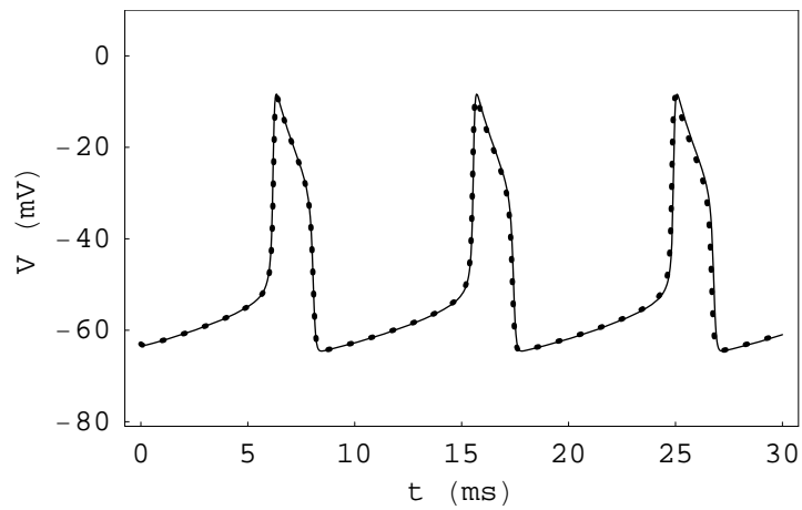
Figure 9: The limit cycle solution of Eqs. (49) - (51) (solid line) may be approximated by the solution of Eqs. (14), (17), (18) and (49) (dotted line) when \beta \gg \delta , and \alpha \gg \gamma . The rate functions \alpha(V) = 6.4 \exp[0.3(V - V_0)/25] , \beta(V) = 17.6 \exp[-1.4(V - V_0)/25] , \gamma(V) = 0.24 \exp[0.345(V - V_0)/25] , \delta(V) = 0.125 \exp[-0.312(V - V_0)/25] , \bar{g}_K = 34 \text{ mS/cm}^2 , \bar{g}_{Na} = 15 \text{ mS/cm}^2 , \bar{g}_L = 0.1 \text{ mS/cm}^2 , V_K = -72 \text{ mV} , V_{Na} = 55 \text{ mV} , V_L = -49.4 \text{ mV} , I = 92 \text{ } \mu\text{A/cm}^2 , V_0 = -57.9 , z_m = 1.3 , V_m = 58 .
