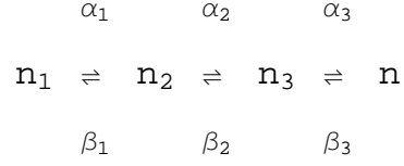
Figure 6: Three-stage activation model of a K^+ ion channel voltage sensor, where the occupation probabilities of the closed states n_1 , n_2 and n_3 and the open state n satisfy a master equation, and \alpha_i , \beta_i for i = 1 to 3 are voltage-dependent rate functions between states.
