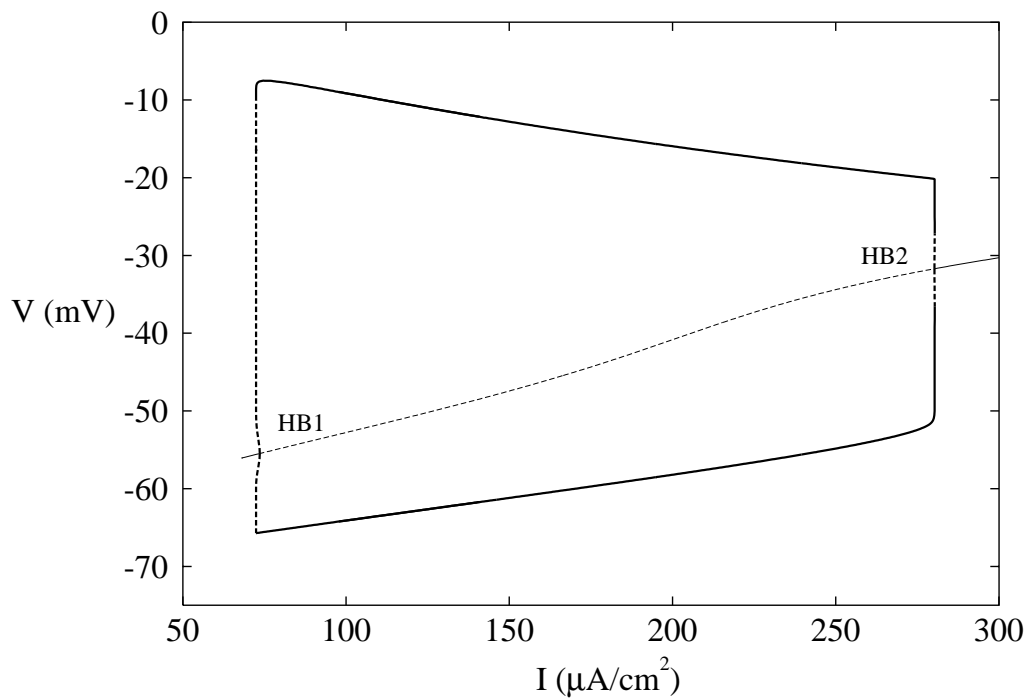
Figure 10: The bifurcation diagram for Eqs. (49) - (51), when \beta \gg \delta and \alpha \gg \gamma , represents the extremal values for the stable periodic solutions (thick solid line), unstable periodic solutions (thick dashed line), and the subcritical bifurcation points HB1 and HB2 at the intersection between stable stationary points (thin solid line) and unstable stationary points (thin dashed line) - see Fig. 9 for a limit cycle solution.
