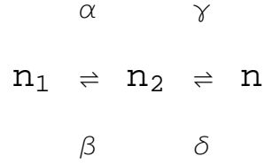
Figure 1: Two-stage activation model of a K^+ ion channel voltage sensor, where the occupation probabilities of the closed states n_1 , n_2 and the open state n satisfy a master equation, and \alpha, \beta, \gamma and \delta are voltage-dependent rate functions between states.
