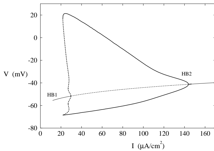
Figure 16: The bifurcation diagram for Eqs. (50) - (51) and Eqs. (55) - (57), when \beta \gg \delta and \alpha \gg \gamma , represents the extremal values for the stable periodic solutions (thick solid line), unstable periodic solutions (thick dashed line) and the subcritical (HB1) and supercritical (HB2) bifurcation points which occur at the intersection between stable stationary points (thin solid line) and unstable stationary points (thin dashed line) - see Fig. 15 for a limit cycle solution.
