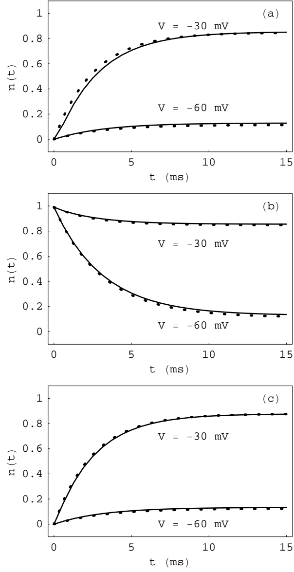
Figure 5: Survival probability of the state n(t) during a voltage clamp for a two-stage model of a K channel (solid line) and HH model (dotted line) during (a) activation and (b) deactivation, for the rate functions of Fig. 4, and (c) activation when \beta(V) and \gamma(V) are increased by a factor of 3, and the rate functions \alpha_H = 0.02(V + 45.8)/(1 - \exp[-0.15(V + 45.8)]) and \beta_H = 0.12 \exp[-0.057(V + 45.8)] .
