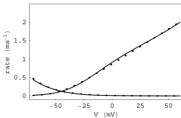
Figure 4: The derived rate functions \alpha_{n,2} and \beta_{n,2} (solid line) in Eqs. (15) and (16) are calculated for the rate functions determined experimentally for the Shaker K^+ ion channel [11] \alpha(V) = 1.1 \exp(0.25V/25) , \beta(V) = 0.37 \exp(-1.6V/25) , \gamma(V) = 2.8 \exp(0.32V/25) , \delta(V) = 0.021 \exp(-1.1V/25) ( \text{ms}^{-1} ), and may be approximated by the rate functions \alpha_H = 0.019(V + 45.8)/(1 - \exp[-0.15(V + 45.8)]) and \beta_H = 0.135 \exp[-0.052(V + 45.8)] for single transition activation (dotted line).
