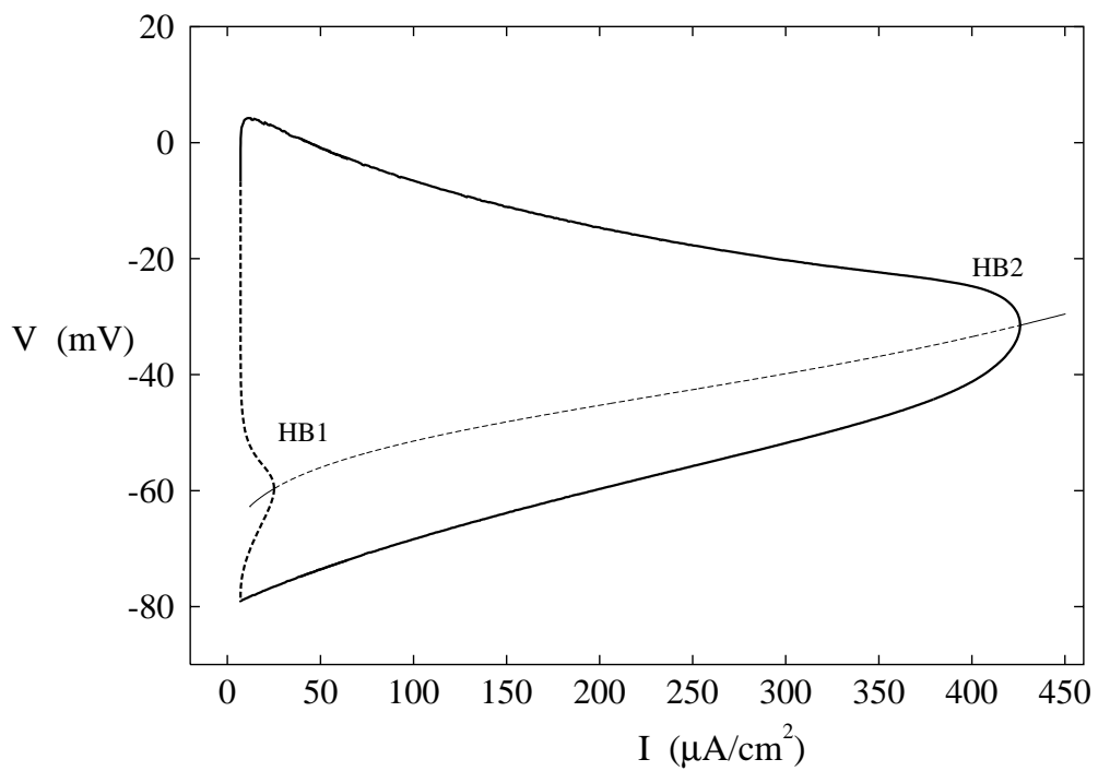
Figure 12: The bifurcation diagram for Eqs. (49) - (51), when \beta \gg \delta and \gamma \gg \alpha , where the subcritical (HB1) and supercritical (HB2) bifurcation points are at the junction between stable stationary points (thin solid line) and unstable stationary points (thin dashed line) - see Fig. 11 for a limit cycle solution.
