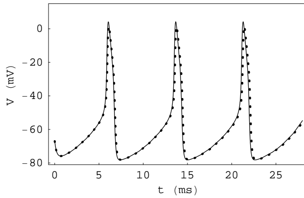
Figure 11: The limit cycle solution of Eqs. (49) - (51) (solid line) may be approximated by the solution of Eqs. (14), (49), (53) and (54) (dotted line) when \beta \gg \delta , and \gamma \gg \alpha . The rate functions \alpha(V) = 1.1 \exp(0.25V/25) , \beta(V) = 1.1 \exp(-1.6V/25) , \gamma(V) = 8.4 \exp(0.32V/25) , \delta(V) = 0.021 \exp(-1.1V/25) , \bar{g}_K = 17 \text{ mS/cm}^2 , \bar{g}_{Na} = 9 \text{ mS/cm}^2 , \bar{g}_L = 0.1 \text{ mS/cm}^2 , V_K = -81 \text{ mV} , V_{Na} = 46 \text{ mV} , V_L = -58.4 \text{ mV} , I = 13 \text{ } \mu\text{A/cm}^2 , z_m = 1.5 , V_m = 51.9 .
