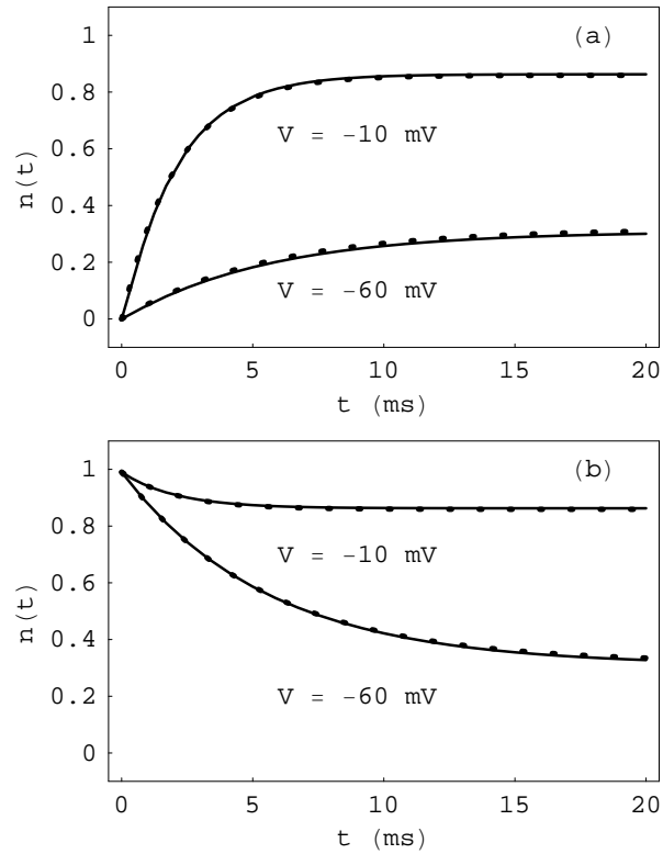
Figure 3: Survival probability of the state n(t) during a voltage clamp for a two-stage activation model of a K^+ ion channel (solid line) and for the HH squid axon model (dotted line) during (a) activation and (b) deactivation (see Fig. 2).
