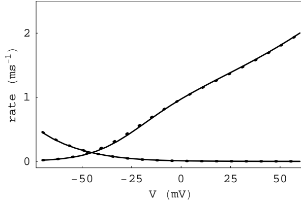
Figure 7: The derived rate functions \alpha_{n,2}(V) and \beta_{n,2}(V) are calculated for a two-stage K^+ channel (solid line), where \alpha(V) = 1.1 \exp(0.25V/25) , \beta(V) = 1.48 \exp(-1.6V/25) , \gamma(V) = 11.2 \exp(0.32V/25) , \delta(V) = 0.021 \exp(-1.1V/25) ( \text{ms}^{-1} ), and \alpha_{n,3}(V) , \beta_{n,3}(V) are calculated for a three-stage K^+ ion channel (dotted line) where the rate functions \alpha_1(V) = 1.1 \exp(0.25V/25) , \alpha_2(V) = 44.8 \exp(0.48 V/25) , \alpha_3(V) = 11.2 \exp(0.32V/25) , \beta_1(V) = 3.0 \exp(-0.7V/25) , \beta_2(V) = 12.0 \exp(-0.7V/25) , \beta_3(V) = 0.021 \exp(-1.1V/25) .
