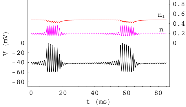
Figure 14: When \beta \ll \delta and \alpha \ll \gamma , Eqs. (49) - (51) may exhibit a small amplitude oscillation in V that alternates with a cluster of spikes, and is described as a bursting oscillation (see Fig. 13).
