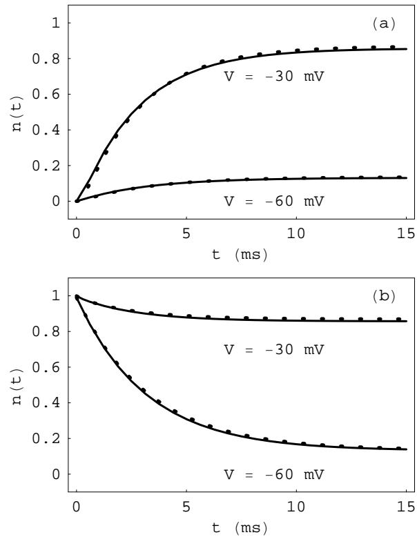
Figure 8: Survival probability of the state n(t) during a voltage clamp for a two-stage (solid line) and three-stage (dotted line) model of activation of a K^+ ion channel voltage sensor during (a) activation and (b) deactivation, for the rate functions of Fig. 7.
