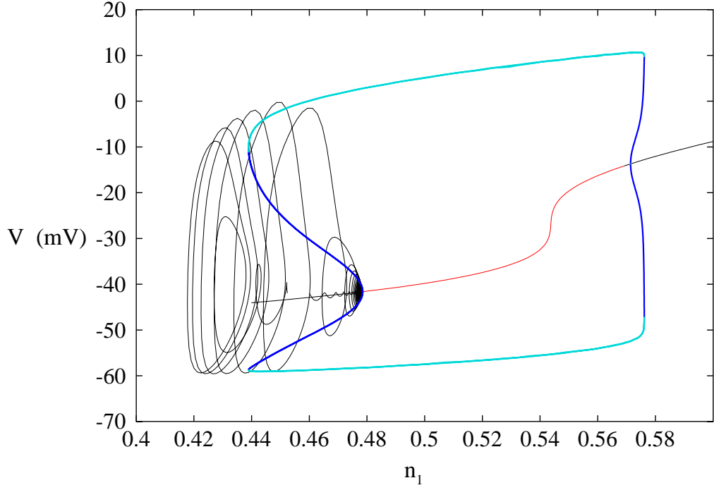
Figure 13: The bifurcation diagram for Eqs. (49) and (50) where \beta \ll \delta and \alpha \ll \gamma , the slow variable n_1 is treated as a parameter in the (V, n) subsystem (red and blue line), and the V vs n_1 projection is computed from Eqs. (49) - (51) (solid line). For n_1 less than 0.48, the stationary point is stable but for n_1 above this value, it is unstable. The rate functions are \alpha(V) = 0.17 \exp(0.5V/25) , \beta(V) = 0.02 \exp(-V/25) , \gamma(V) = 2.8 \exp(0.45V/25) , \delta(V) = 0.44 \exp(-V/25) , \alpha_m(V) and \beta_m(V) defined by Eq. (52), V_m = 45 , \bar{g}_K = 36 mS/cm 2 , \bar{g}_{Na} = 12 mS/cm 2 , \bar{g}_L = 0.4 mS/cm 2 , V_K = -90 mV, V_{Na} = 70 mV, V_L = -70 mV, I = 236 \mu A/cm 2 .
