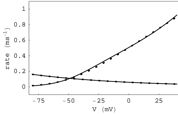
Figure 2: The derived rate functions \alpha_{n,2} and \beta_{n,2} (solid line) in Eqs. (17) and (18) provide a good approximation to the HH rate functions ( \text{ms}^{-1} ) \alpha_n = 0.01(V + 50)/[1 - \exp(-0.1(V + 50))] and \beta_n = 0.125 \exp[-(V + 60)/80] (dotted line) when the rate functions for two-stage activation ( \text{ms}^{-1} ) are \alpha(V) = 6.4 \exp[0.3(V - V_0)/25] , \beta(V) = 17.6 \exp[-1.4(V - V_0)/25] , \gamma(V) = 0.24 \exp[0.345(V - V_0)/25] , \delta(V) = 0.125 \exp[-0.312(V - V_0)/25] , V_0 = -57.9 .
