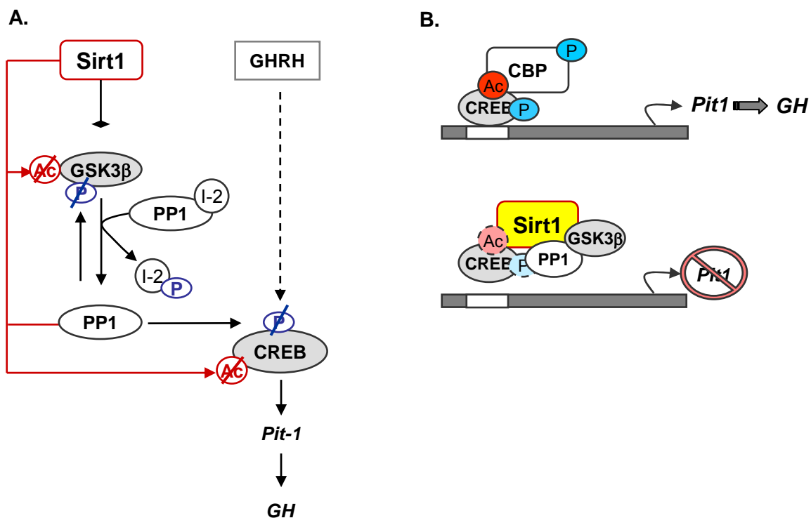
Figure 31. A. Schematic presentation of the signaling events taking place after Sirt1 activation, according to the findings of the present work. Sirt1 intercepts the cAMP pathway downstreams to GHRH (dotted line) at CREB level. Sirt1 physically associates with GSK3 \beta , PP1 and CREB (red line). Sirt1 activation deacetylates and activates GSK3 \beta . The activated GSK3 \beta phosphorylates the PP1 inhibitor I-2, releasing it from the PP1 complex. This leads to the suppression of the inhibitory Ser 9 phosphorylation and further activation of GSK3 \beta via an autoregulatory loop. The free active PP1 associates with CREB and dephosphorylates it, while Sirt1 deacetylates it. The de-phosphorylated and de-acetylated CREB loses its transcriptional activity so there is less Pit1 transcription, which compromises the sufficient GH synthesis.
