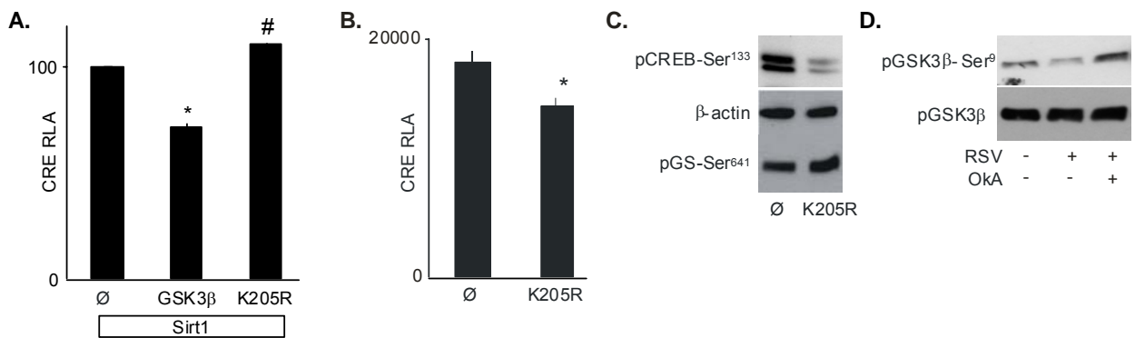
Figure 30. A. CRE transcriptional activity in GH3 cells transfected with Sirt1 in the presence of GSK3β and mutated GSK3β K205R. B. CRE transcriptional activity in GH3 cells transfected with mutant GSK3β K205R. RLA: relative luciferase activity. Luciferase was measured 24 hours after transfection. Results are shown as luciferase:β-galactosidase ratio. Each experiment was repeated twice. *P<0.001 to empty plasmid control (Ø); # P<0.05 to empty plasmid control. C. pCREB-Ser 133 and pGS-Ser 641 levels in GH3 cells transfected with GSK3β K205R. The same membrane was used and reblotted after sequential strippings. D. Effect of 2 hour pretreatment with 10nM okadaic acid (OkA) on resveratrol's suppressive effect on GSK3β-Ser 9 . Immunoblots were repeated twice.
