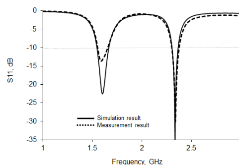
Fig. 2 Reflection coefficient of CP patch antenna
