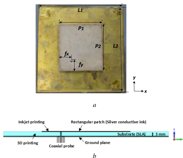
Fig. 1 Circularly polarised patch antenna geometry
