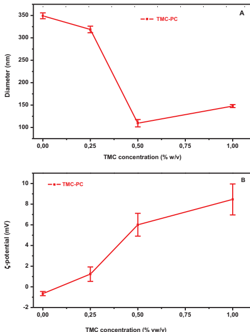
Fig. (1). The effect of different TMC concentration on (A.) the size of TMC-coated liposomes in PBS pH 7.4, (B.) the \zeta -potential of TMC-coated liposomes in PBS pH 7.4. The results are the mean of three different experiments.
