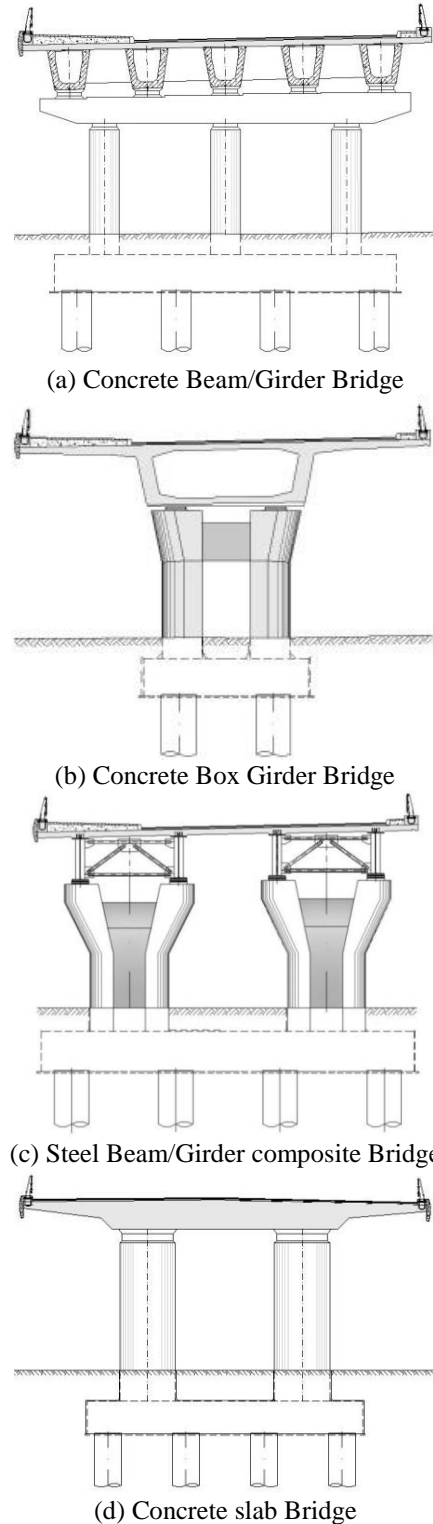
Figure 1 SeeBridge Bridge Types
