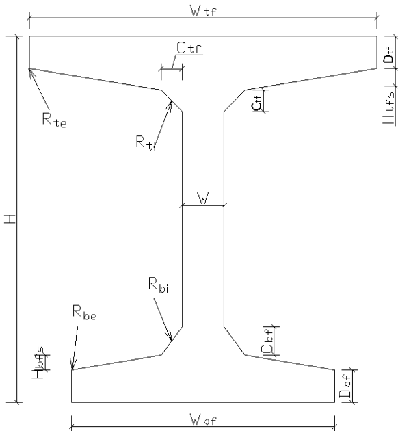
Figure 4 SeeBridge generic girder parametric cross-section
