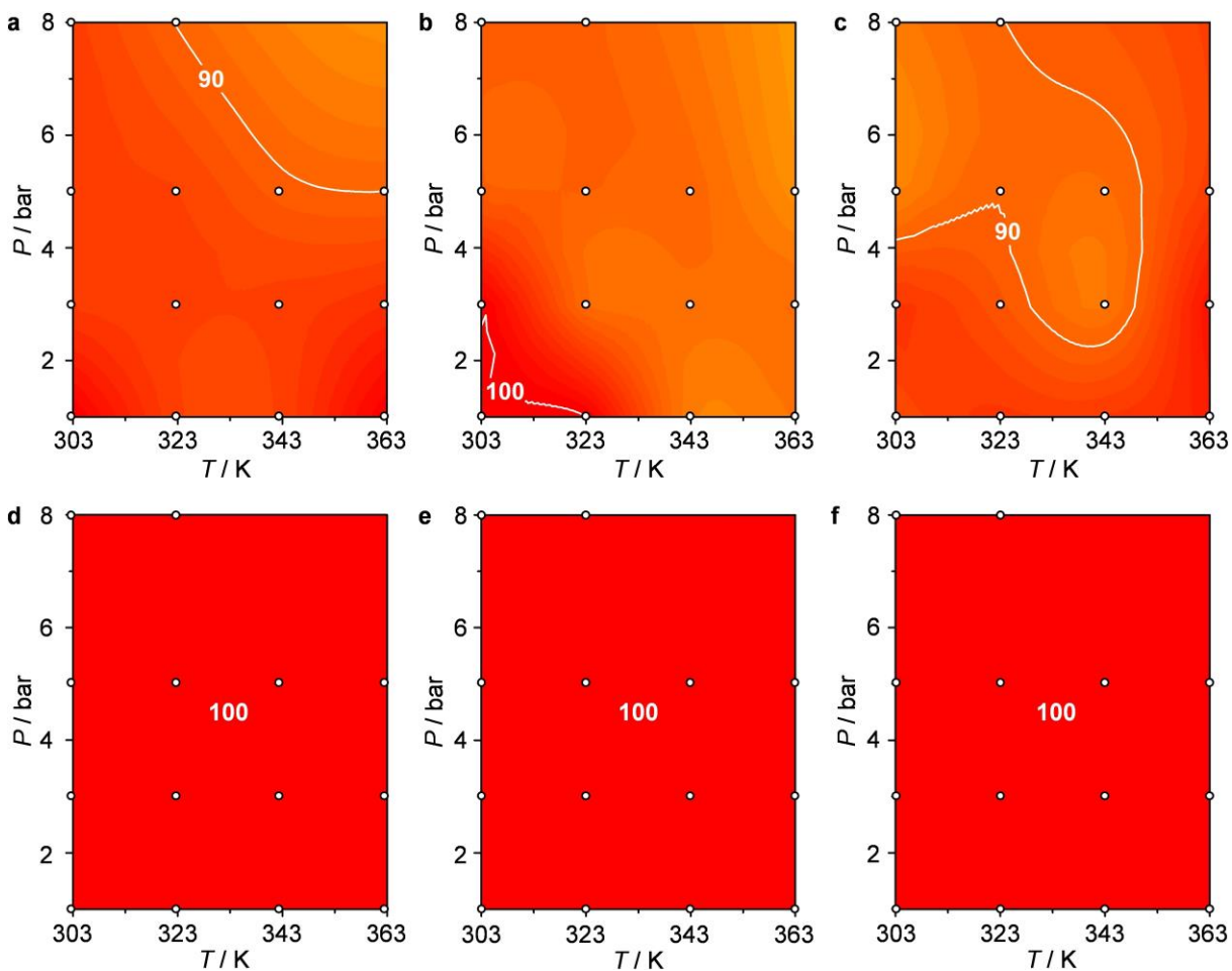
Figure S16. Selectivity (in %) to 1-hexene at different temperatures and total pressures over a) Pd-BCN-P1, b) Pd-MCN-0.5-P1, c) Pd-MCN-P1, d) Pd-BCN-D2, e) Pd-MCN-D1 and f) Pd-MCN-D2. Reaction conditions: W_{\text{cat}} = 0.1 \text{ g} , F_L(1\text{-hexyne+toluene}) = 1 \text{ cm}^3 \text{ min}^{-1} and F_G(\text{H}_2) = 36 \text{ cm}^3 \text{ min}^{-1} . The contour maps were obtained through spline interpolation of 14 experimental points.
