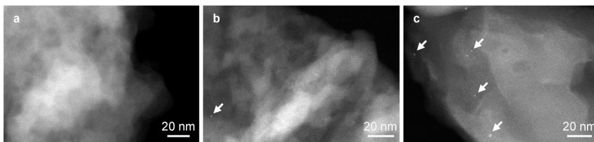
Figure S6. STEM HAADF images of a) Ir-MCN-P1, b) Ir-ECN-P1 and c) Ir-BCN-P1. The arrows in b,c) indicate the nanoparticles.
