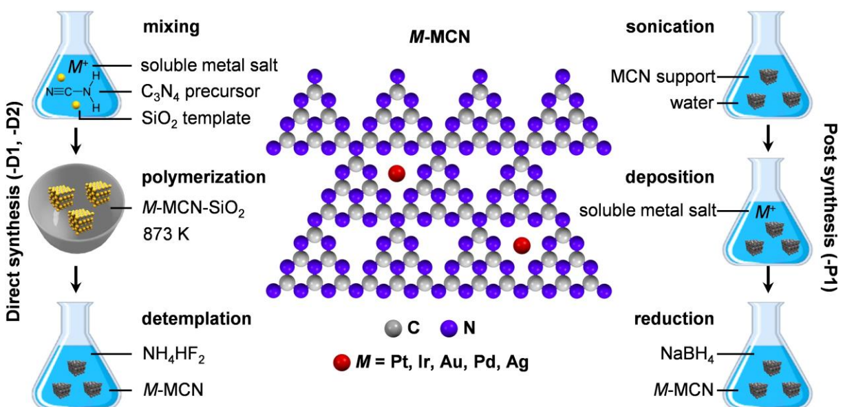
Figure 1. Direct synthesis (-D1, -D2) and post-synthesis (-P1) approaches to stabilize metal atoms within g- C_3N_4 , exemplified for the mesoporous MCN carrier. In the idealized location depicted, the metal atom is coordinated by up to 6 nitrogen atoms within interstices defined by the packing of the tri-s-triazine units.
