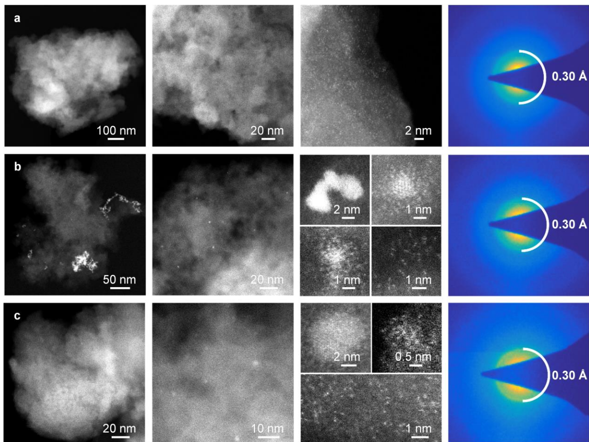
Figure S8. AC-STEM HAADF images and diffraction patterns of selected M -MCN systems prepared by post-synthetic routes: a) Ir-MCN-P1, b) Pt-MCN-P1 and c) Pd-MCN-P1.
