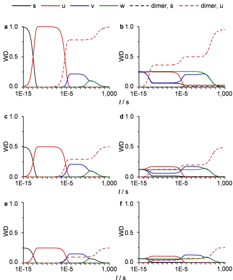
Figure S11. KMC simulations of the impact of the initial metal concentration and distribution on the stabilization of Pt atoms in g\text{-C}_3\text{N}_4 . Kinetic profiles of the weight distributions (WD) of Pd species arising from a,b), a 25% initial occupancy of all sites simulated at 300 K. Similar set ups with c,d), a half and e,f), a quarter the amount of atoms in a,b). In a,c,e), the surface layer is completely occupied and all other sites are vacant while in b,d,f), the same amount of atoms is distributed uniformly among all sites.
