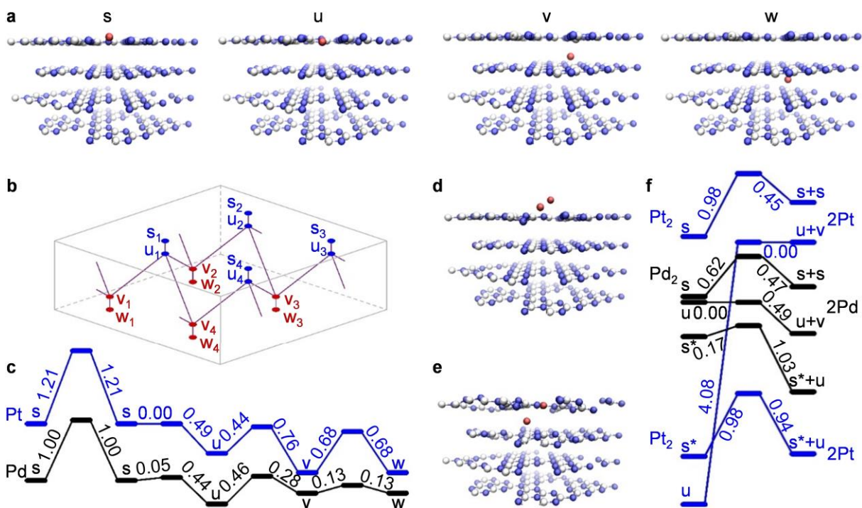
Figure 6. a) DFT optimized incorporation of metal atoms in g-C 3 N 4 ( M = \text{red} , \text{C} = \text{white} , \text{N} = \text{blue} ), showing the four identified equilibrium positions of metal atoms. Two are located slightly above (s) and below (u) the six-fold cavities between the tri-s-triazine units in the surface g-C 3 N 4 layer, and another two are found above (v) and below (w) the six-fold cavities in the subsurface g-C 3 N 4 layer. Some C and N atoms have been hidden to facilitate visualization of the metal. b) Identified transition paths of metal atoms inside the surface and sub-surface layers of g-C 3 N 4 , c) corresponding energy profiles for translocation of Pt and Pd atoms along these paths, d,e) identified equilibrium positions of metal dimers above d) and below e) the surface layer of g-C 3 N 4 , f) energy profiles for the association of metal dimers and their decomposition into pairs of atoms located in neighboring s+s, s * +u, or u+v positions (s * denotes s-sites occupied by hydrogenated, thus, immobile metal atoms or dimers).
