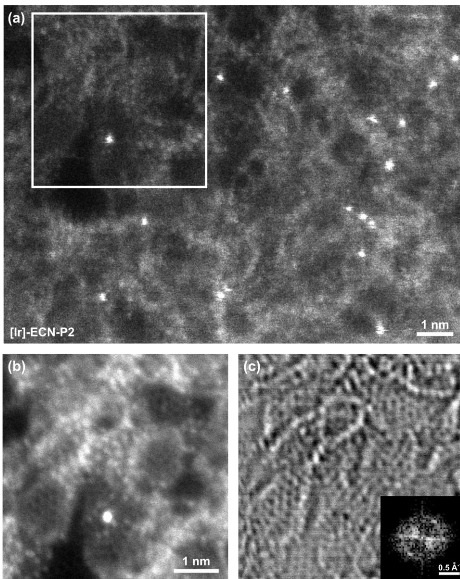
Figure 4. ‘Gentle STEM’ analysis of a model Ir SAHC. a) Atomically resolved STEM HAADF image showing Ir atoms distributed across the ECN support, b) simultaneous STEM HAADF and c) BF images of the boxed region in a). The inset in c) is a local Fourier transform taken from the lower left hand region of the image. These images are a sum of 50 frames acquired rapidly over approximately 50 s and summed to produce images with high contrast and clarity. The very bright dot in b) is a single Ir atom anchored on a g-C 3 N 4 raft.
