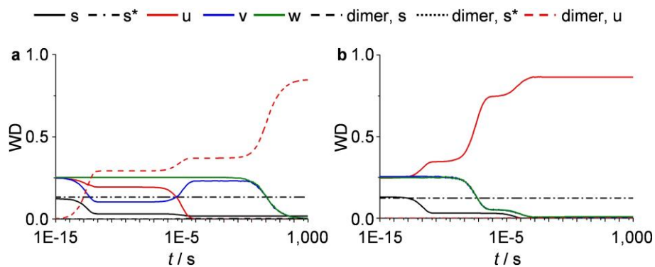
Figure S13. KMC simulations illustrating the impact of hydrogen on the stabilization of a) Pt and b) Pd atoms in g\text{-C}_3\text{N}_4 . In all cases 50% of the atoms are hydrogenated in the initial state and thus fixed in their positions, while 50% are free to move. The metal atoms in the initial state are uniformly distributed between all sites.
