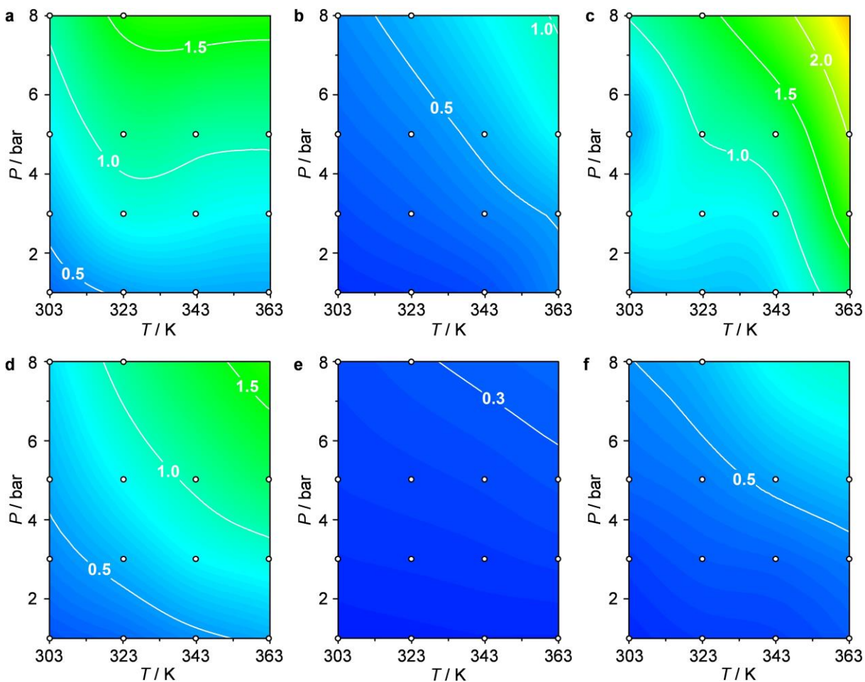
Figure 8. Reaction rate of 1-hexyne hydrogenation (in 10^3 \text{ mol}_{1\text{-hexene}} \text{ mol}_{\text{Pd}}^{-1} \text{ h}^{-1} ) at different temperatures and pressures over a , Pd-BCN-P1; b , Pd-MCN-0.5-P1, c , Pd-MCN-P1, d , Pd-BCN-D2, e , Pd-MCN-D1 and f , Pd-MCN-D2. The contour maps were obtained through spline interpolation of 14 experimental points. Reaction conditions: W_{\text{cat}} = 0.1 \text{ g} , F_L(1\text{-hexyne+toluene}) = 1 \text{ cm}^3 \text{ min}^{-1} and F_G(\text{H}_2) = 36 \text{ cm}^3 \text{ min}^{-1} .
