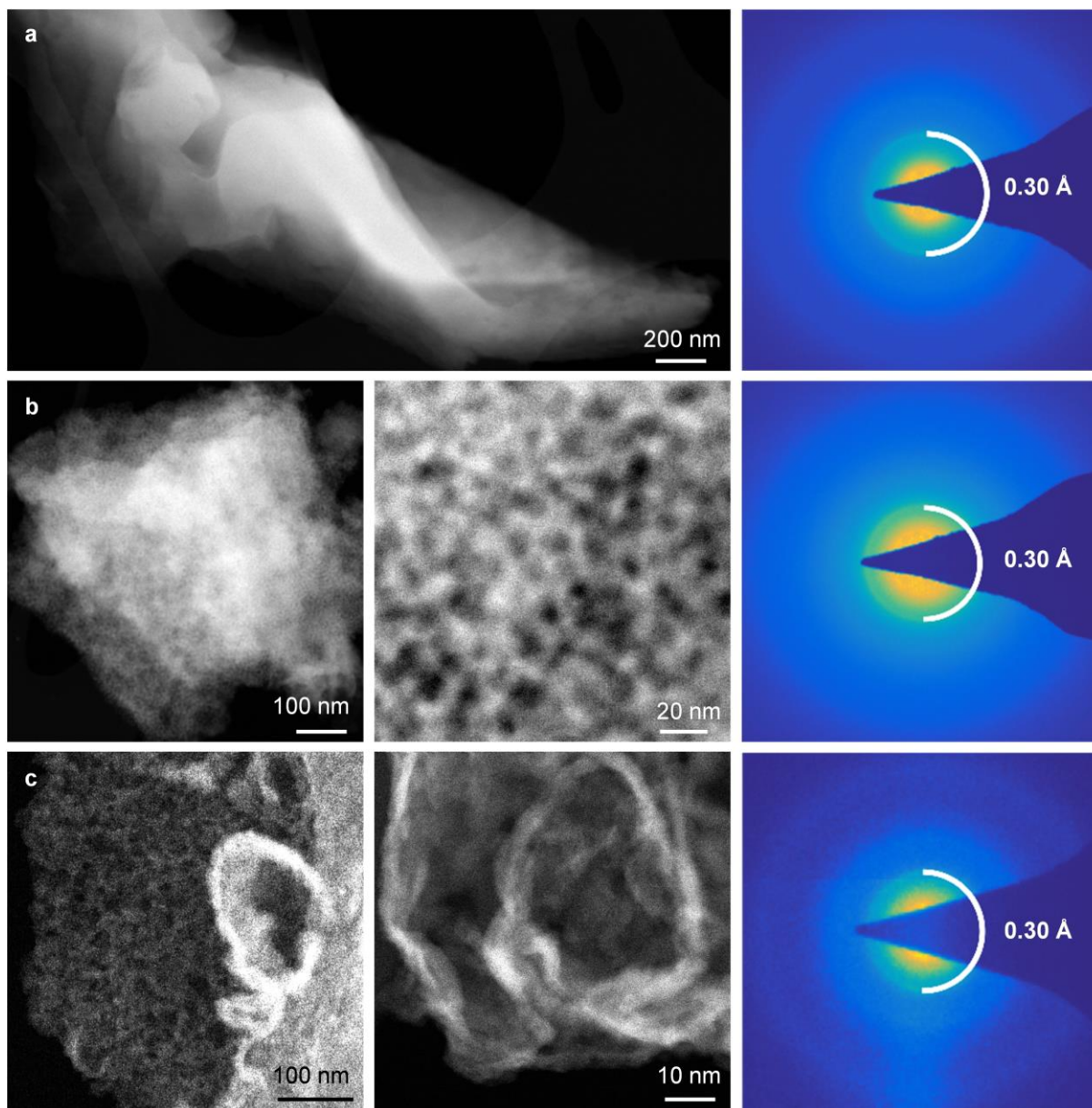
Figure S2. Additional STEM HAADF TEM images and diffraction patterns of a) BCN, b) MCN and c) ECN.
