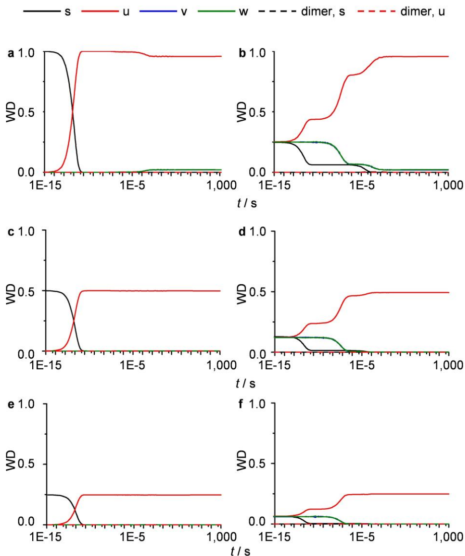
Figure S12. KMC simulations of the impact of the initial metal concentration and distribution on the stabilization of Pd atoms in g-C 3 N 4 . Kinetic profiles of the weight distributions (WD) of Pd species arising from a,b), a 25% initial occupancy of all sites simulated at 300 K. Similar set ups with c,d), a half and e,f), a quarter the amount of atoms in a,b). In a,c,e), the surface layer is completely occupied and all other sites are vacant while in b,d,f), the same amount of atoms is distributed uniformly among all sites.
