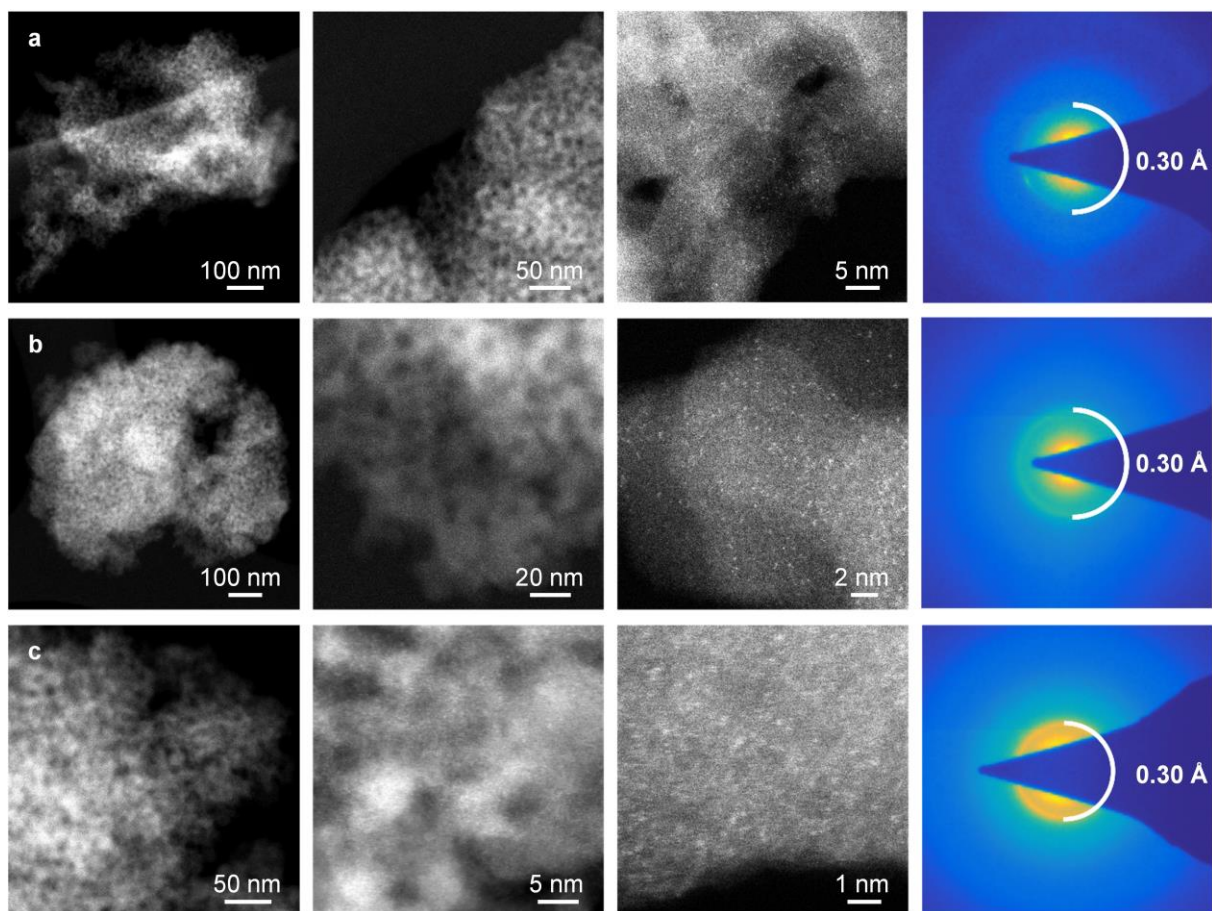
Figure S7. AC-STEM HAADF images and diffraction patterns of selected M -MCN systems prepared by direct synthesis: a) Ir-MCN-D1, b) Pt-MCN-D1 and c) Ag-MCN-D2.
