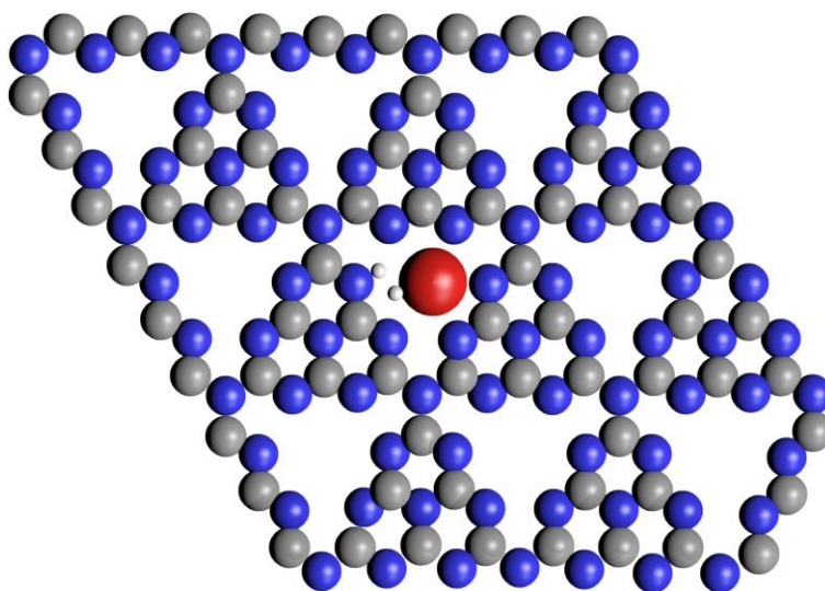
Figure S14. Idealized structure of a Pd atom isolated at an s position in g\text{-C}_3\text{N}_4 interacting with two H atoms. Color codes: Pd = red, C = gray, N = blue, H = white.
