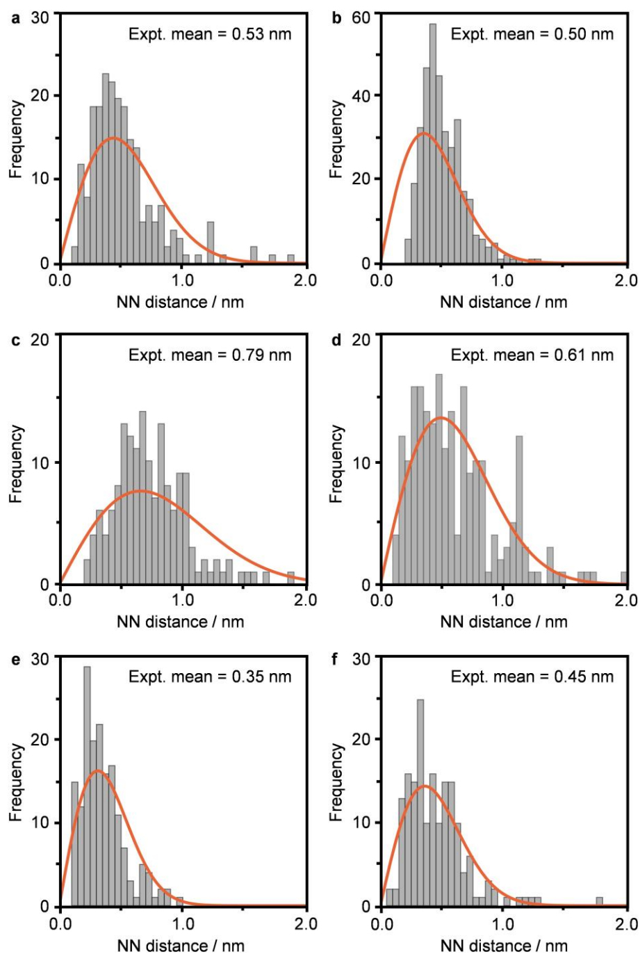
Figure S9. Measured nearest neighbor (NN) distances between metal atoms in a) Ir-MCN-D1, b) Ir-MCN-P1, c) Pt-MCN-D1, d) Pt-MCN-P1, e) Pd-MCN-P1 and f) Ag-MCN-D1. Although the three-dimensional structure of the supports means that two well-separated metal atoms at different heights may appear very close in projection, a good agreement with the distribution expected for a randomly dispersed set of points in an equivalent area (red curves) is observed in all cases.
