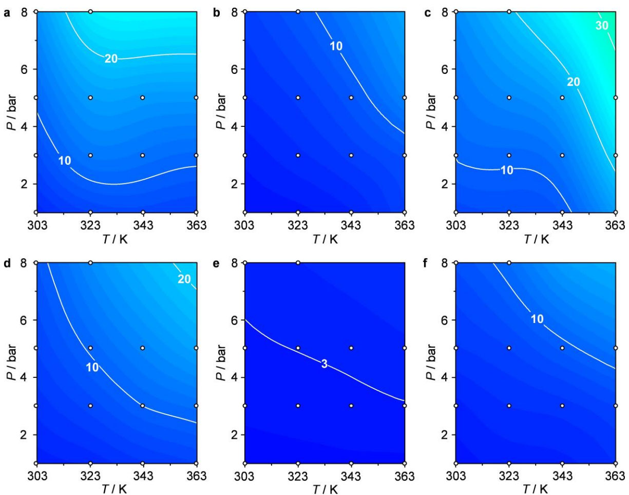
Figure S15. Conversion (in %) of 1-hexyne at different temperatures and total pressures over a) Pd-BCN-P1, b) Pd-MCN-0.5-P1, c) Pd-MCN-P1, d) Pd-BCN-D2, e) Pd-MCN-D1 and f) Pd-MCN-D2. Reaction conditions: W_{\text{cat}} = 0.1 \text{ g} , F_L(1\text{-hexyne+toluene}) = 1 \text{ cm}^3 \text{ min}^{-1} and F_G(\text{H}_2) = 36 \text{ cm}^3 \text{ min}^{-1} . The contour maps were obtained through spline interpolation of 14 experimental points.
