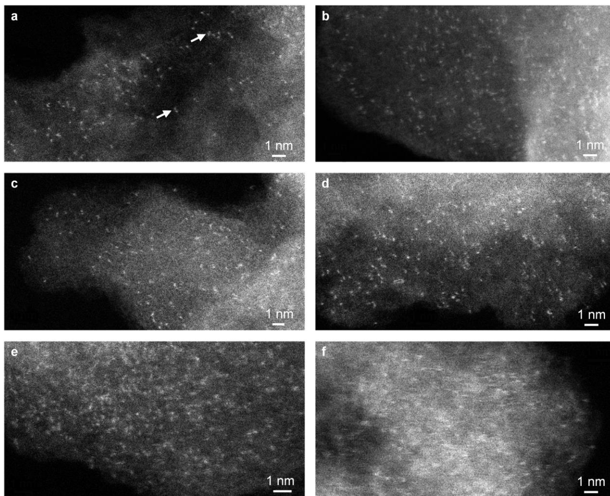
Figure S5. Atomically resolved AC-STEM HAAD images of selected SAHCs: a) Ir-MCN-D1, b) Ir-MCN-P1, c) Pt-MCN-D1, d) Pt-MCN-P1, e) Pd-MCN-P1 and f) Ag-MCN-D1. The arrows in a) indicate examples of pairs of atoms in close proximity suggesting dimerization.
