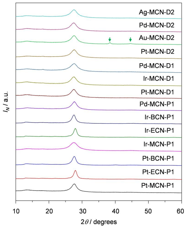
Figure S4. Normalized XRD patterns of all the metal-containing samples.
