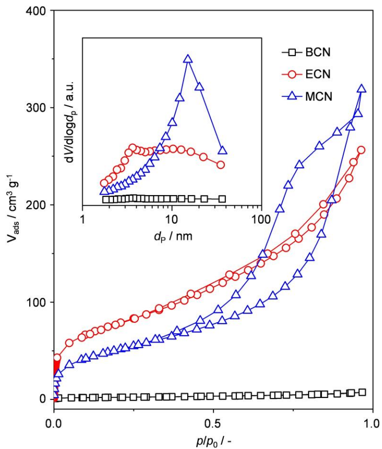
Figure S1. Argon isotherms and corresponding Barrett-Joyner-Halenda mesopore size distributions (inset) of the g-C 3 N 4 carriers
