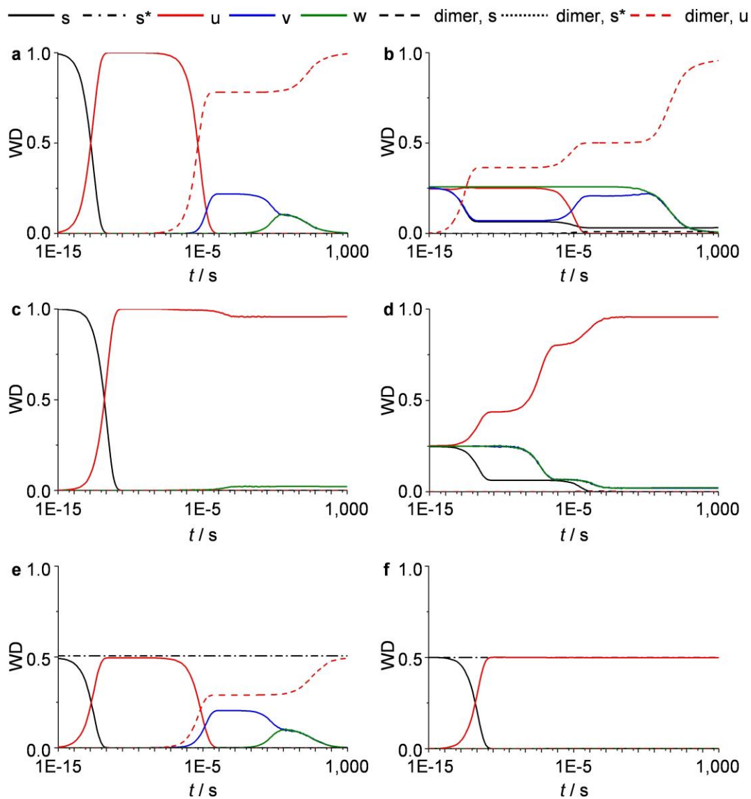
Figure 7. KMC simulations at 300 K comparing the weight distribution (WD) of different a,b) Pt and c,d) Pd species with time. In the first simulations a,c), all s sites are occupied by atoms in the initial state, which are free to move during the simulation, other sites are vacant. In the second simulations b,d) the same amount of atoms is initially distributed uniformly between all sites. KMC simulations illustrating the impact of hydrogen on the stabilization of e) Pt and f) Pd atoms in g\text{-C}_3\text{N}_4 . In all cases 50% of the atoms are hydrogenated in the initial state and thus fixed in their positions, while 50% are free to move. The metal distribution in the initial state only occupies the s-sites.
