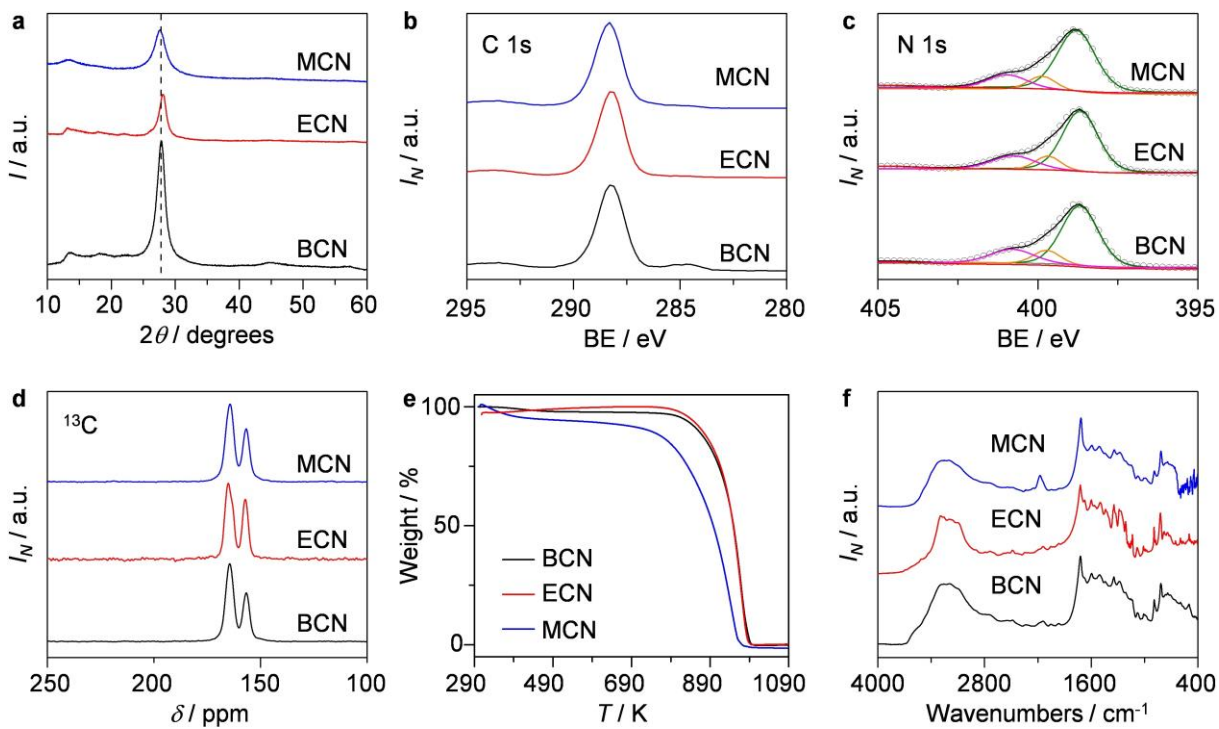
Figure S3. a) XRD patterns, b,c) C 1s and N 1s XPS spectra, d) 13 C CP/MAS NMR spectra, e) TGA profiles and f) DRIFTS spectra of the g-C 3 N 4 carriers.
