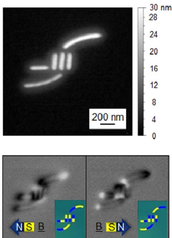
43 Figure 21. Topography (top) and phase shift (bottom) MFM images of the NAND/NOR 44 gates fabricated by the merging of NWs. The phase shift images evidence the magnetic 45 reversal of the gates by applying an external magneticfield in opposite directions (arrows 46 directions), whereas the inlays in panel a, show the magnetic dipole orientations where blue 47 and yellow represent north and south poles, respectively. Reprinted with permission from M. 48 Gavagnin, H. D. Wanzenboeck, D. Belic and E. Bertagnolli, "Synthesis of individually tuned 49 nanomagnets for nanomagnet logic by direct write focused electron beam induced 50 deposition", ACS Nano, 7, 777-784, (2013). Copyright 2012 American Chemical Society. 51 52 53 54 55 56 57 58 59 60
