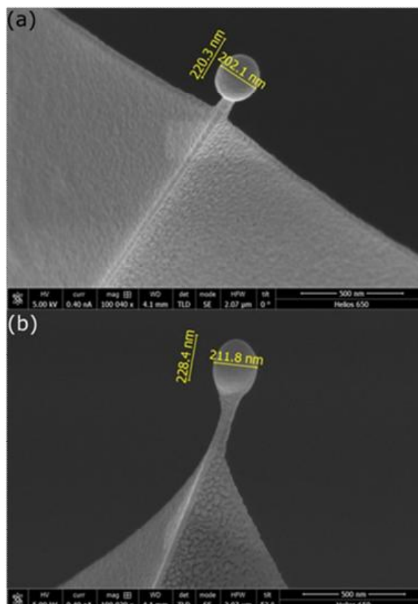
42 Figure 13. (a, b) Scanning electron micrographs of Co nanospheres of 200 nm in diameter 43 44 grown at the tip of soft cantilevers used for Ferromagnetic Resonance Force Microscopy. 45 46 47 48
