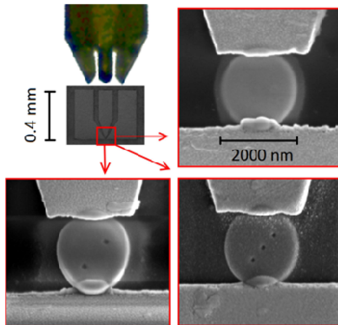
30 31 32 33 34 35 36 37 38 39 40 41 42 43 44 45 Figure 20. The top left panel shows an optical image of the high frequency probe and the gold contacts to which it is attached. The other three panels show SEM images of the Co dots deposited by FEBID between the gold contacts. Three cases are shown: without nanoholes, with two nanoholes, and with three nanoholes. Reprinted with permission from A. Lara et al., Applied Physics Letters 105, 182402 (2014). Copyright [2014], AIP Publishing LLC.
