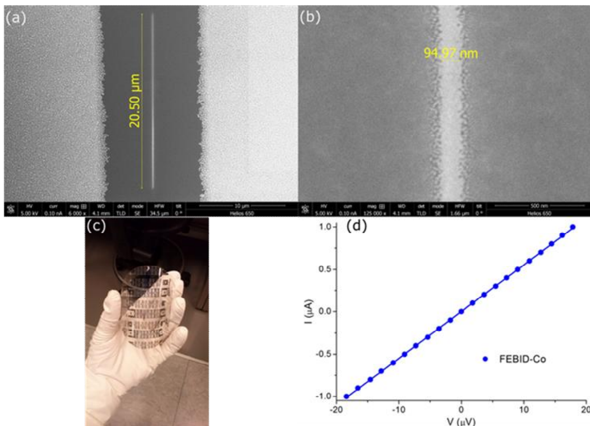
36 37 Figure 9. (a, b) Scanning electron micrographs of Co nanowires grown by FEBID on 38 flexible and transparent polycarbonate substrates. (c) Picture of a polycarbonate substrate 39 patterned by means of optical lithography to allow electrical measurements. (d) Current vs 40 voltage characteristic of a Co nanowire grown by FEBID on polycarbonate. Reproduced 41 with permission from P. Peinado et al., ACS Nano, 2015, 9(6), 6139-6146. Copyright (2015) 42 American Chemical Society. 43 44 45 46 47 48 49 50 51 52
