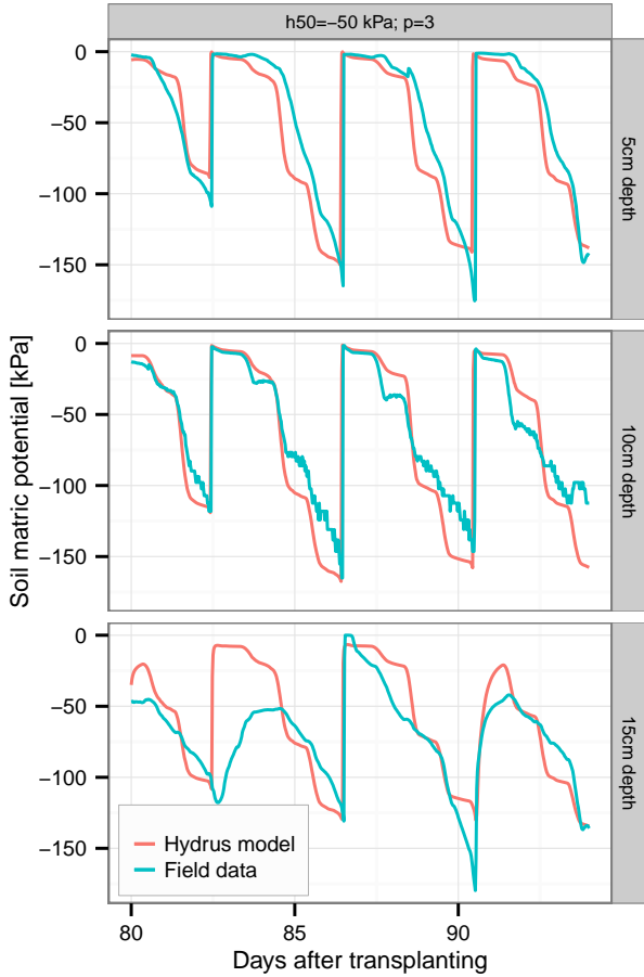
Figure 4: Comparison between modeled and measured SMP for T66low at 5, 10 and 15 cm depth from 80 to 94 DAT for the best set of parameters.
