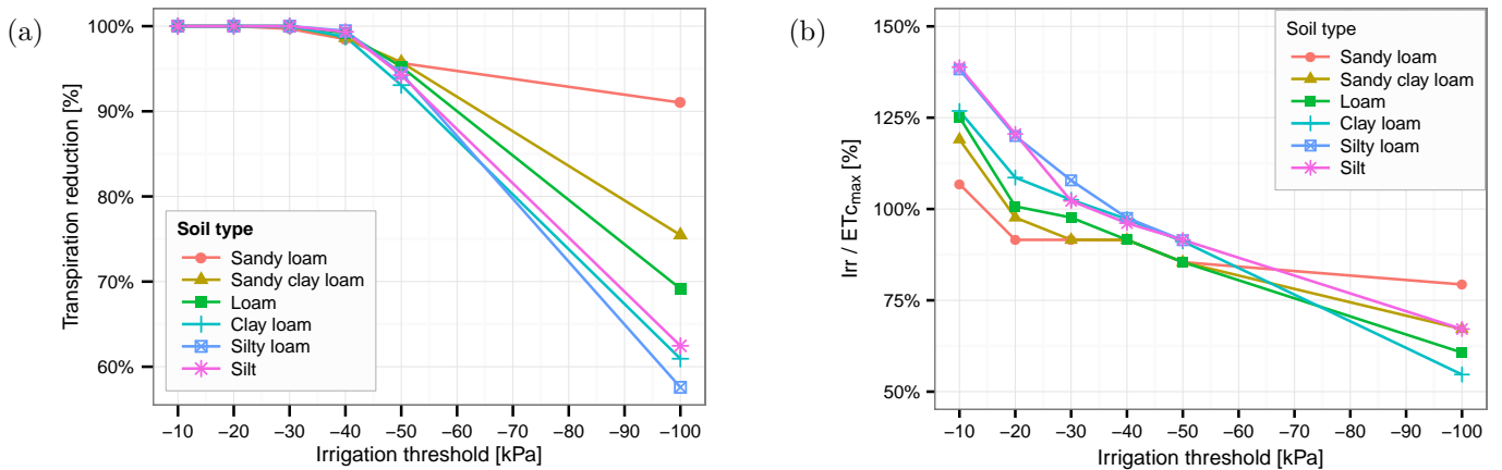
Figure 7: (a) Ratio of actual over maximal transpiration; (b) ratio of cumulative irrigation amounts ( Irr ) over cumulative maximal crop evapotranspiration ( ET_{c,max} ) for the mid-season, and for different soil textures.
