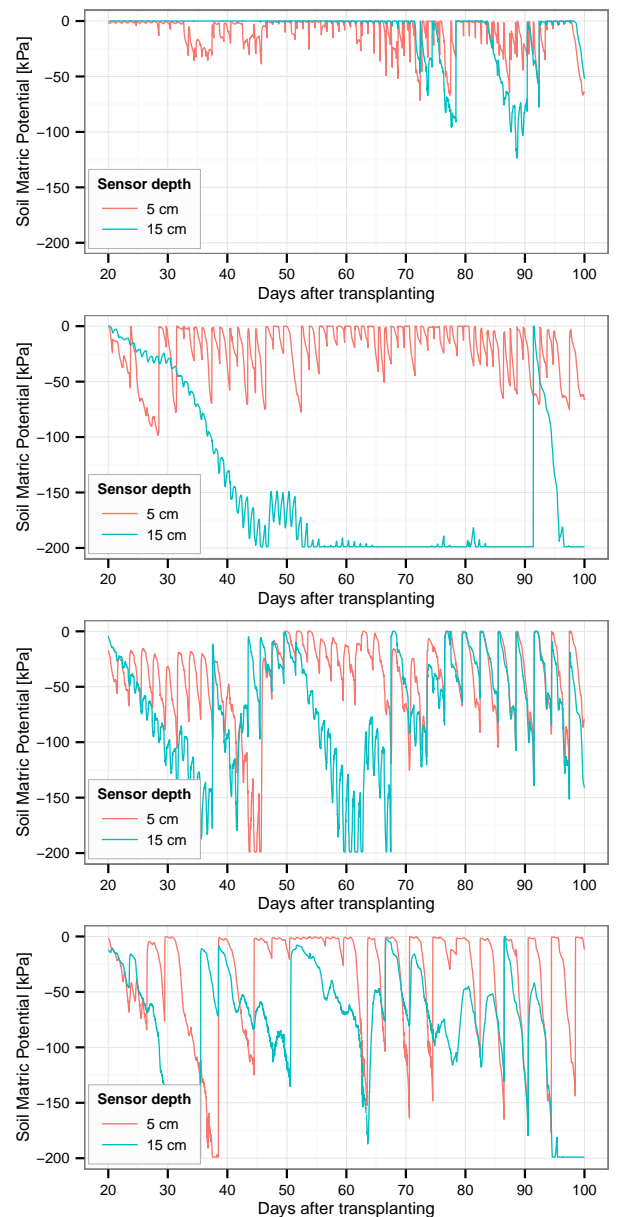
Figure 1: Evolution of the soil matrix potential for T150low, T66low, T100high, T66high (top to bottom) for sensors at 5 and 15 cm depth, 12 cm away from a microtube.
