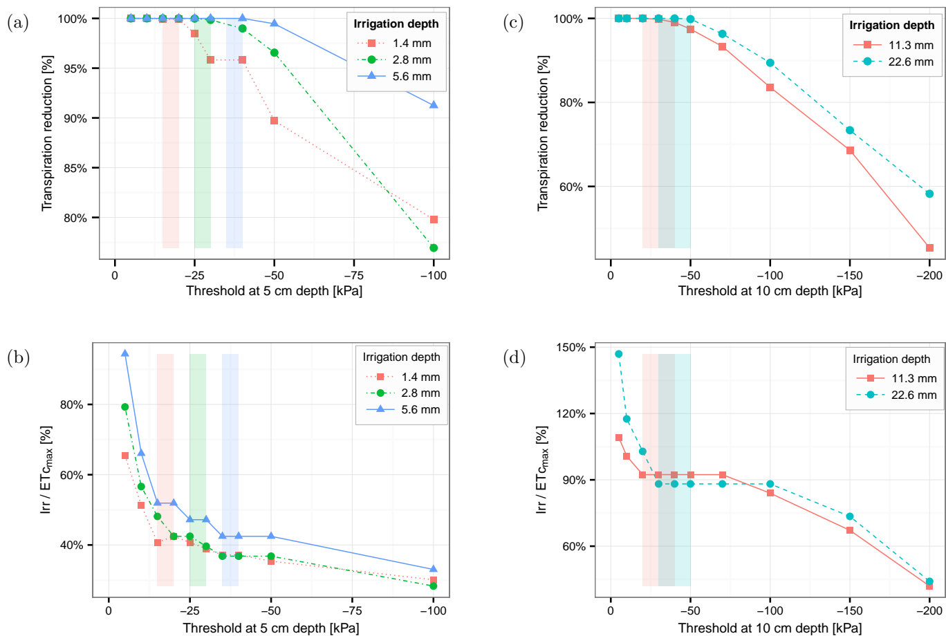
Figure 5: Results of all scenarios for varying irrigation thresholds at 5 cm depth for the early growth stage and 10 cm depth for the mid-season and for different irrigation depth. (a) and (b) represent scenarios for the early growth stage (10-30 DAT); (c) and (d) show the results for the mid-season (60-80 DAT); (a) and (c) show the simulated cumulative actual transpiration volumes over the cumulative maximal transpiration amounts. (b) and (d) represent the reduction in irrigation water applied to the crop, using the ratio of cumulative irrigation amounts ( Irr ) to the cumulative amounts of maximal crop evapotranspiration ( ET_{cmax} ). The colored ribbons show the regions of optimal thresholds given the irrigation depth (higher value avoids water losses, lower value limits transpiration reduction).
