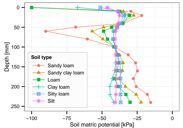
Figure 8: SMP distribution with depth just before an irrigation event for a threshold of -40 kPa at 10 cm depth.
