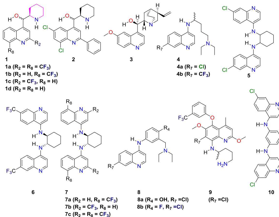
Figure 1. Structural formulae of known and novel antimalarials described in this study, wherein 1a represents mefloquine (cycloaliphatic piperidinyl ring highlighted in magenta), 2 (6, 8-Dichloro-2-phenyl-quinolin-4-yl)-piperidin-2-yl-methanol, 3 quinine, 4a chloroquine, 5 , 6 , 7 without additional letters are used generically to describe any isomer. There are two isomers for these three compounds named as -trans (R-R) with trans geometry, and -cis (R,S) with cis geometry, with the identifiers equatorial (eq) and axial (ax), respectively, referring to the position of the substituent amino nitrogen atoms relative to the cyclohexane ring. 8a represents amodiaquine, 9 WR 238,605 (Tafenoquine) [17] and 10 metaquine. [23]
