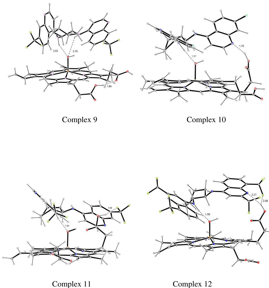
Figure 13. DFT optimized structures of complexes 9, 10, 11 and 12 with distances in Å. Hydrogen bonds shown as dotted lines
