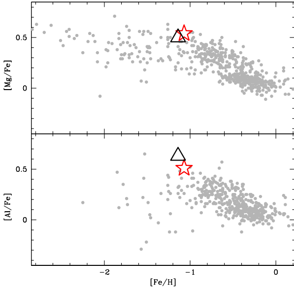
Figure 3. Upper panel: [\text{Mg}/\text{Fe}] vs [\text{Fe}/\text{H}] trends for NGC 6362 (red star) and M 4 (black triangle), compared to a sample of field stars (grey dots). Lower panel: same comparison for [\text{Al}/\text{Fe}] .
