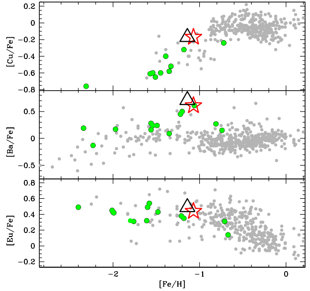
Figure 6. Upper panel: [\text{Cu}/\text{Fe}] vs [\text{Fe}/\text{H}] trends for a sample of Galactic GCs (green circles) taken from (Simmerer et al. 2003), a sample of thick disk stars taken from (Reddy et al. 2003; Reddy, Lambert, & Allende Prieto 2006) and the cluster under analysis. Central panel: observed Ba trends for the same populations (data for the 14 plotted GCs have been taken from D’Orazi et al. 2010). Lower panel: same comparison but for Eu abundances.
