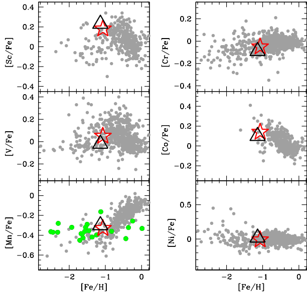
Figure 5. Comparison among the trends of the iron-peak element abundances vs. [\text{Fe}/\text{H}] as measured for NGC 6362, M 4 and field stars. Green circles indicate the [\text{Mn}/\text{Fe}] average abundances derived by (Sobeck et al. 2006) for 21 Galactic GCs.
