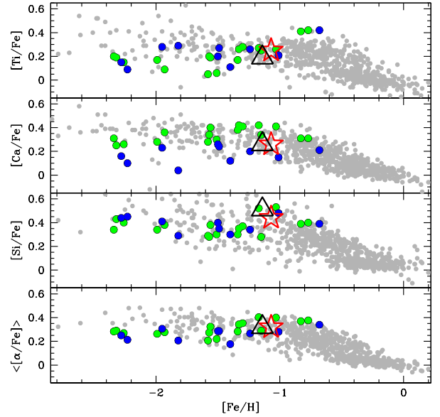
Figure 4. Upper three panels: [\text{Si}/\text{Fe}] , [\text{Ca}/\text{Fe}] , [\text{Ti}/\text{Fe}] vs. [\text{Fe}/\text{H}] trends for NGC 6362, field stars (same symbols of Figure 3) and Galactic GCs (green circles are taken from Carretta et al. 2009, blue circles from Mészáros et al. 2015). Lower panel: same comparison on the \langle[\alpha/\text{Fe}]\rangle vs. [\text{Fe}/\text{H}] trend. NGC 6362 is in very good agreement with what observed for the other GCs.
