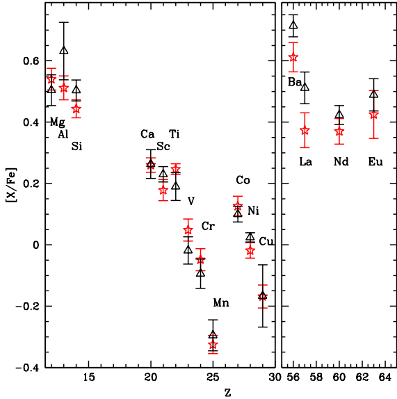
Figure 7. Comparison among the elemental abundances measured for NGC 6362 (red star symbols) and M 4 (black triangles).
