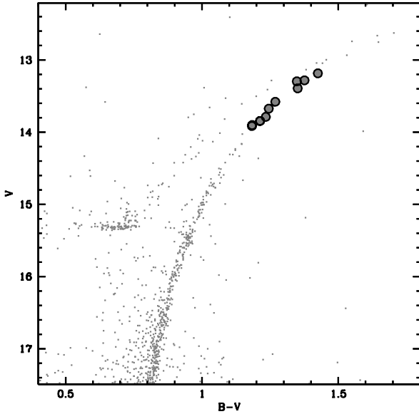
Figure 1. Optical (V, B-V) CMD of NGC 6362 in the innermost 300'' (the photometry comes from the catalogue described in Dalessandro et al. 2014 ). The UVES targets are highlighted with black filled circles.
