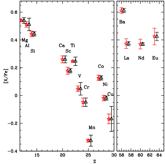
Figure 8. Comparison among the elemental IQR for NGC 6362 (red bars) and M 4 (black bars). For sake of comparison, all the pairs are plotted at the same y-axis value (that measured for NGC 6362).
