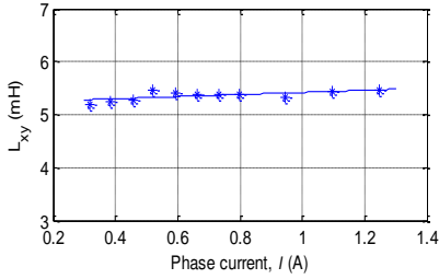
Fig. 13. Inductance obtained from the x-y plane excitation.
