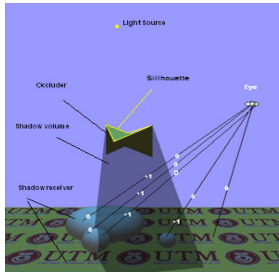
Figure 6: Shadow volume using stencil buffer and depth buffer
