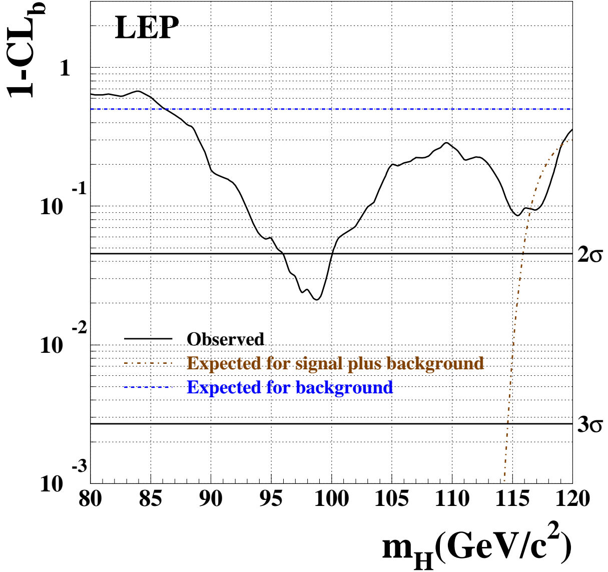
Figure 7: The background confidence 1 - CL_b as a function of the test mass m_H . Full curve: observation; dashed curve: expected background confidence; dash-dotted line: the position of the minimum of the median expectation of 1 - CL_b for the signal plus background hypothesis, when the signal mass indicated on the abscissa is tested. The horizontal solid lines indicate the levels for 2\sigma and 3\sigma deviations from the background hypothesis (see the Appendix for the conversion).
