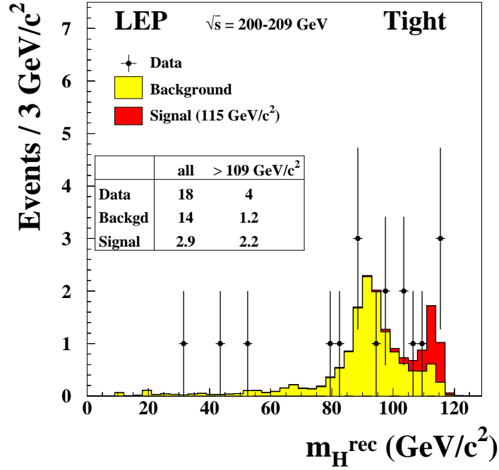
Figure 5: Distributions of the reconstructed Higgs boson mass, m_H^{\text{rec}} , obtained from two selections with differing signal purities. The histograms show the Monte Carlo predictions, lightly shaded for the background, heavily shaded for an assumed Standard Model Higgs boson of mass 115 GeV/c 2 , together with the data. In the loose and tight selections the cuts are adjusted in such a way as to obtain, for a Higgs boson of mass 115 GeV/c 2 , approximately 0.5 or 2 times more expected signal than background events when integrated over the region m_H^{\text{rec}} > 109 GeV/c 2 . In the searches where the event selection depends on the test mass (see the Appendix), its value is set at 115 GeV/c 2 .
