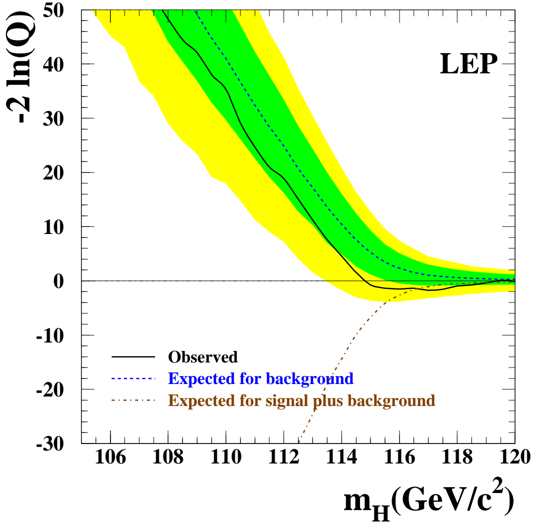
Figure 1: Observed and expected behaviour of the test statistic -2\ln Q as a function of the test mass m_H , obtained by combining the data of the four LEP experiments. The full curve represents the observation; the dashed curve shows the median background expectation; the dark and light shaded bands represent the 68% and 95% probability bands about the median background expectation. The dash-dotted curve indicates the position of the minimum of the median expectation for the signal plus background hypothesis when the signal mass given on the abscissa is tested.
