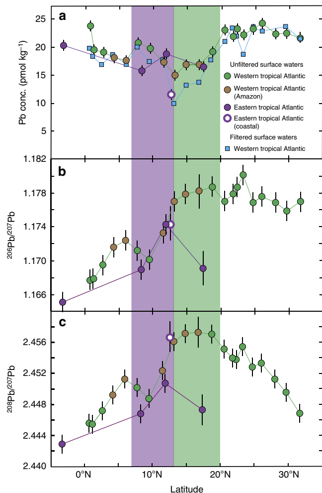
Figure 2 | Lead concentrations and isotopic compositions results for surface seawater samples. Panel (a) displays Pb concentration results, while panels (b) and (c) display ^{206}\text{Pb}/^{207}\text{Pb} and ^{208}\text{Pb}/^{207}\text{Pb} ratios respectively, as a function of latitude. Circles denote the results for unfiltered seawater samples, and squares are results for filtered seawater (western Tropical Atlantic only). Green and purple shaded fields denote the position of the North African dust plume during the 64PE321 and D361 cruise, in the western and eastern Tropical Atlantic (WTA and ETA) respectively. Uncertainty assessed through replicate analyses of in-house seawater standards quoted at 1 s.d. for Pb concentrations and 2 s.d. for Pb isotope ratios 66 .
