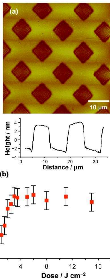
Figure 2. (a) AFM height image of a dry micropatterned PCysMA brush layer obtained after UV exposure ( \lambda = 244 \text{ nm} ) of a brominated initiator surface through a mask followed by ATRP, together with a representative line section. A dry, unpatterned brush prepared under identical conditions had a thickness of 7 nm. (b) Variation in brush height difference between masked and exposed regions of micropatterned brushes as a function of UV dose during patterning.
