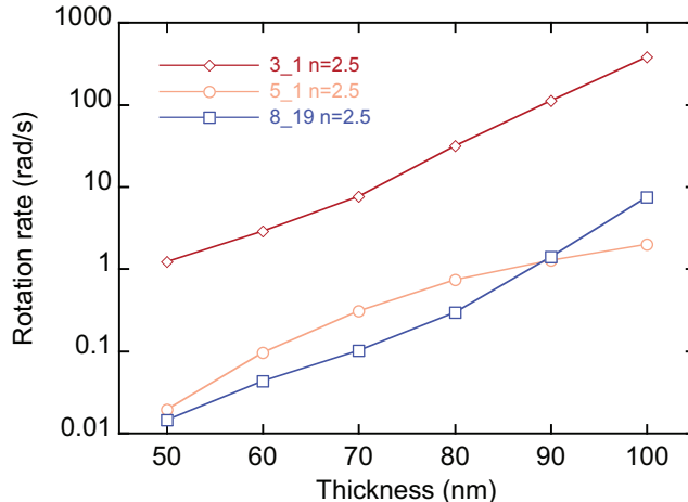
Figure 2. The rotation rates of knots of type 3_1 , 5_1 and 8_{19} in counter-propagating circularly polarised plane waves.
