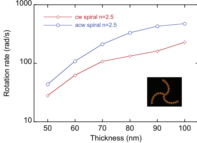
Figure 3. The rotation rates for 3-armed spirals with two different chiralities. The structure is shown in the inset. The modulus of rotation rate is plotted, but the rotation rates for the anti-clockwise spiral (blue trace) should be negative with respect to the clockwise spiral (red trace).
