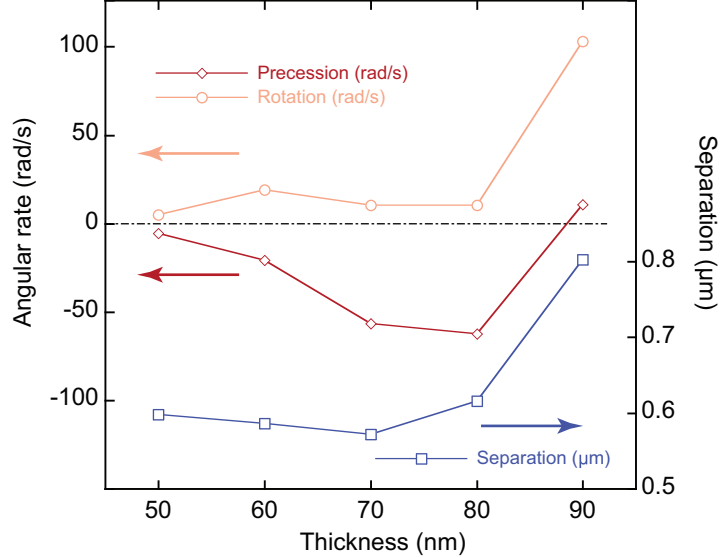
Figure 4. Rotation and precession rates, and binding separations, for pairs of 3_1 knots of various thicknesses.
