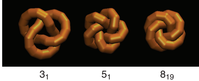
Figure 1. Schematic showing the three knotted nanowires used throughout this paper. In the simulations, the knotted nanowires are oriented so that the faces shown are perpendicular to the propagation direction. i.e. the plane of the diagram corresponds to a bright interference fringe.
