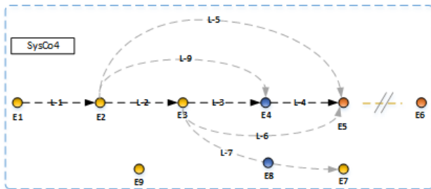
Figure 7 - SysCo4
