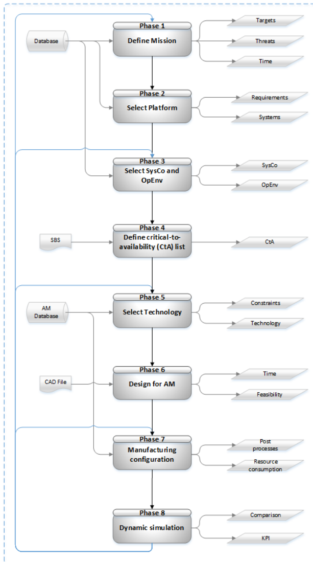
Figure 20 - Framework
