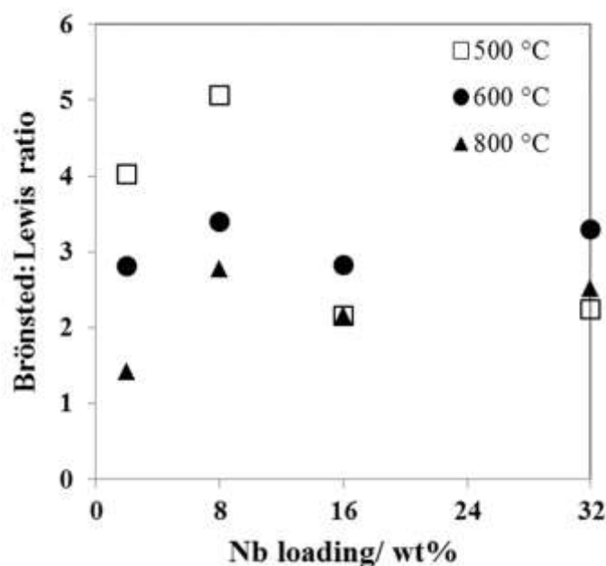
Figure 6. The correlation between Nb loading ( x = 2 to 32 wt%) and the B/L ratio in samples xNb/SBA-15 calcined at 500, 600 and 800 °C.
