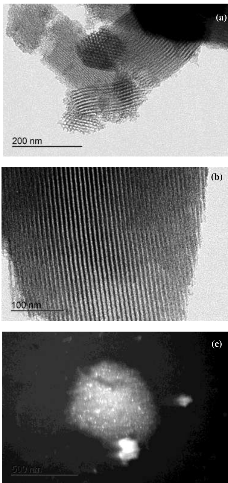
Figure 4. Bright-field TEM images of (a) parent SBA-15, and (b) 2Nb/SBA-15(500) and (c) dark-field STEM image of 2Nb/SBA-15(500).
