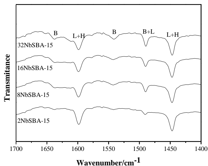
Figure 5. DRIFT spectra of pyridine adsorption over xNb/SBA-15(y) (y = calcined at 500 °C) as a function of Nb loading (x = 2 to 32 wt%).
