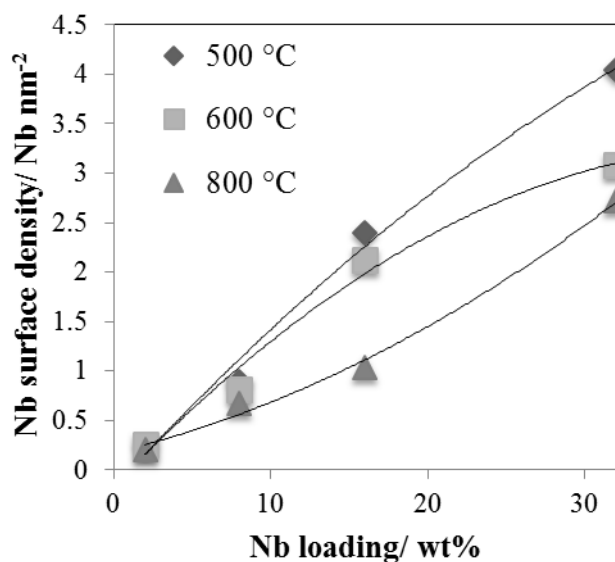
Figure 3. Evolution of Nb surface density with Nb content as a function of calcination temperature for xNb/SBA-15 (x = 2 to 32 wt%).
