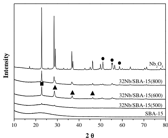
Figure 2. XRD patterns of 32Nb/SBA-15 as a function of calcination temperature. A reference pattern for commercial pure \text{Nb}_2\text{O}_5 is shown, and reflections associated with pseudo-hexagonal (TT, ▲), orthorhombic (T, ■) and monoclinic ( \alpha , ●) niobia indicated.
