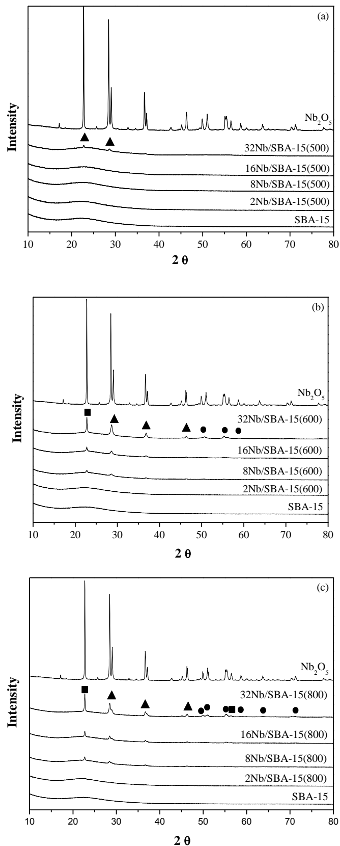
Figure 1. XRD patterns of Nb/SBA-15 as a function of Nb loading and calcination temperature: (a) 500 °C; (b) 600 °C and (c) 800 °C. A reference pattern for commercial pure Nb 2 O 5 is shown, and reflections associated with pseudo-hexagonal (TT, ▲), orthorhombic (T, ■) and monoclinic (α, ●) niobia indicated.
