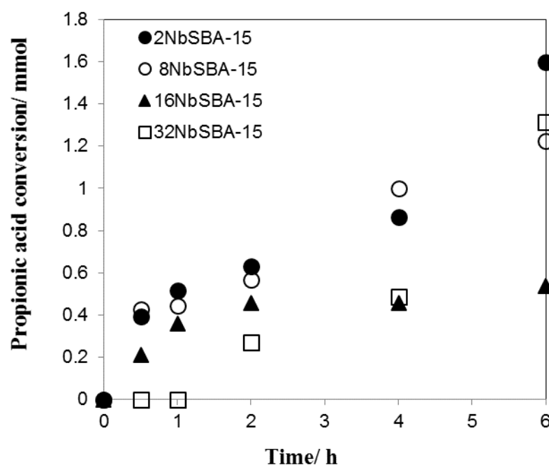
Figure 7. Conversion profiles for the esterification of propionic acid with methanol catalyzed by xNb/SBA-15 ( x = 2 to 32 wt%) calcined at 500 °C. Reactions conditions: 10 mmol of propionic acid, molar ratio MeOH/acid = 30, 50 mg of catalyst and 60 °C.
