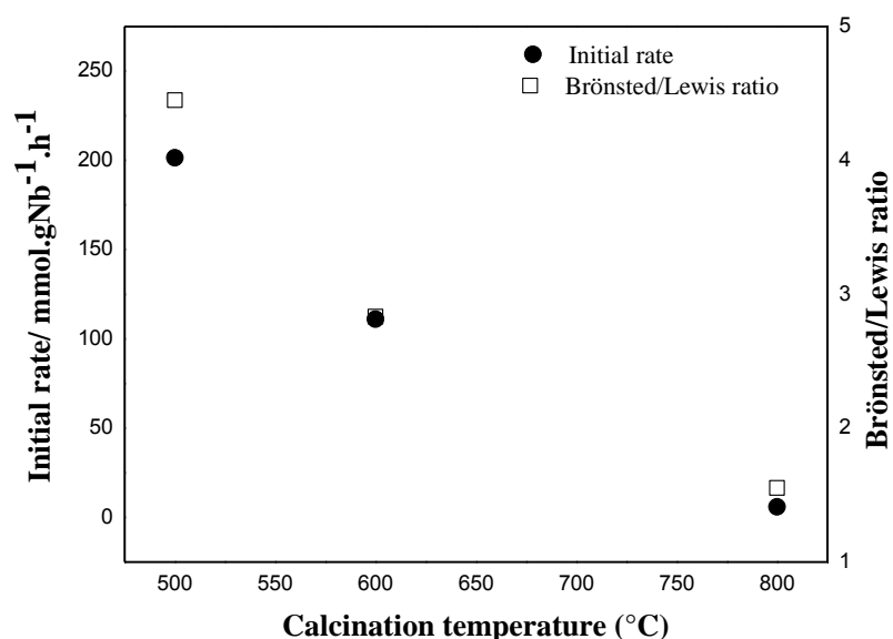
Figure 9. Correlation between initial rate, Nb loading and B/L ratio for the solids catalysts prepared xNb/SBA-15(y) (x = 2 wt %, y = 500, 600 and 800 °C).
