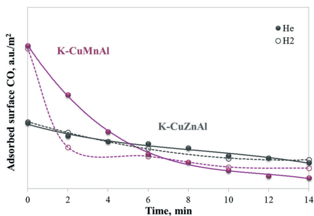
Fig. 8 Amount of surface CO species as a function of time after 3% CO/He adsorption followed by flushing in He (solid lines) or 6% \text{H}_2 /He (dotted lines) over K-CuZnAl and K-CuMnAl.
