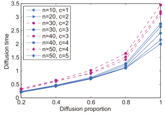
Fig. 4. Performance under different n and c .
