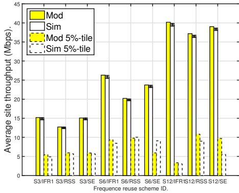
(b) Mean site throughput (Mbps).
