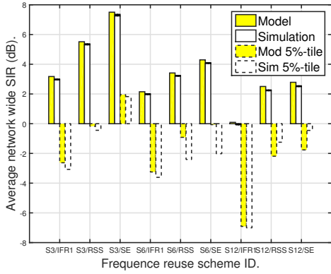
(a) Mean SIR (dB).
