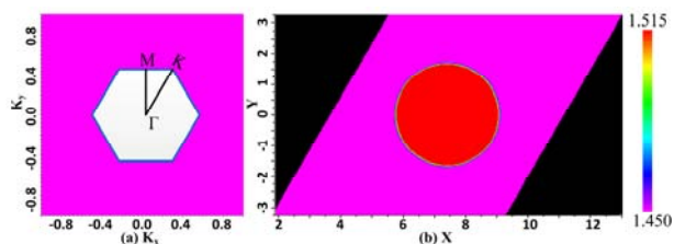
Fig. 3. (a) First Brillouin zone and k-path for a hexagonal lattice. (b) Index profile for the single unit cell.
