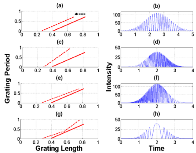
Fig. 2. Comparison between redistribution of local Bragg wavelength in the sensing grating (dashed lines) with respect to the reference grating (solid lines) for (a) uniform, and (c), (e) and (g) non-uniform strains applied. Figures (b), (d), (f) and (h) show the resulting temporal waveforms.
