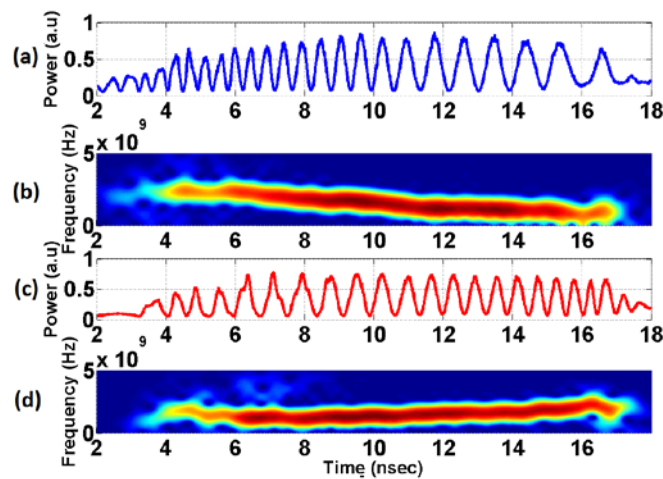
Fig. 5. Demonstration of nonuniform strain sensing. (a, c) The measured temporal waveforms, and (b, d) their spectrograms for nonuniform expansion and compression of the sensing LCFBG, respectively.
