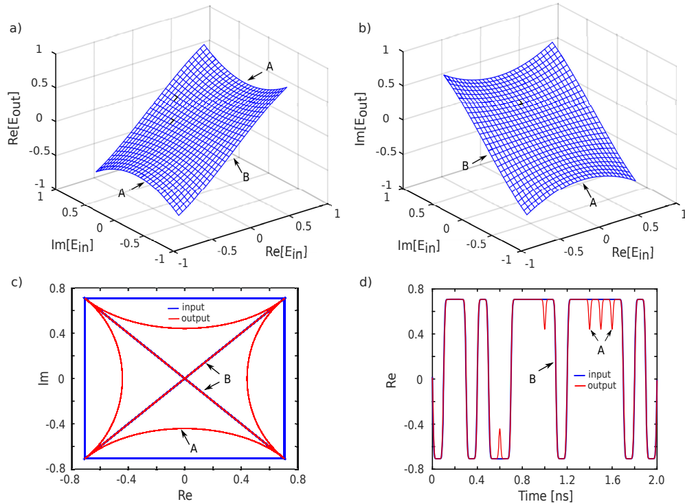
Fig. 2. PSA response in Cartesian coordinates. Specifically, (a) depicts the real part, and (b) the imaginary part of the output signal E_{\text{out}} , as a function of the complex coordinates of the input signal E_{\text{in}} . The power of the output signal has been normalized with respect to the gain of the PSA. (c) Constellation of QPSK signal at the PSA input (in blue) and corresponding output (in red). Substantial trajectory changes noticed for horizontal or vertical transitions, whereas diagonal transitions remain the same. (d) Corresponding time domain waveforms of real signal quadrature at the PSA input (in blue) and output (in red).
