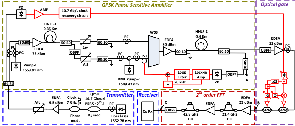
Fig. 4. Experimental setup of proposed PSA-based QPSK 3R regenerator.
