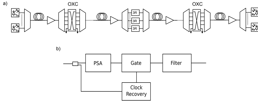
Fig. 1. (a) Schematic of a physical layer transmission path from a typical DWDM network system that employs 3R regenerators and optical cross-connects. (b) Block diagram of proposed 3R regenerator architecture.
