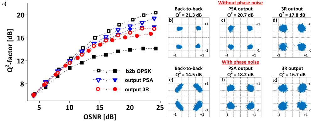
Fig. 6. (a) Q^2 -factor measured at the input of the 3R regenerator and the outputs of the PSA stage and the retiming stage as a function of the OSNR degradation at the receiver: open symbols represent system performance without input phase noise and solid symbols with phase noise. Constellation diagrams of received signal: (b) at the input, (c) at the PSA (2R) output and (d) at the 3R output without input phase distortion, respectively; (e) at the input, (f) at the PSA (2R) output and (g) at the 3R output with input phase distortion.
