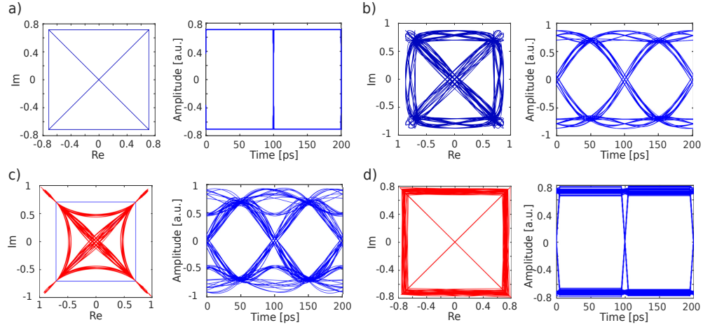
Fig. 3. Constellation and corresponding eye diagrams of the QPSK signal waveform: (a) at the input of the transmission system; (b) at the input of the PSA after strong spectral narrowing accumulated by the transmission process; (c) at the PSA output showing the achieved suppression of the phase distortion at the alphabet points, but also the inability of the PSA to correct the signal waveform during symbol transitions; (d) at the output of the 3R regenerator, demonstrating elimination of the timing uncertainty and recovery of the initial pulse shape.
