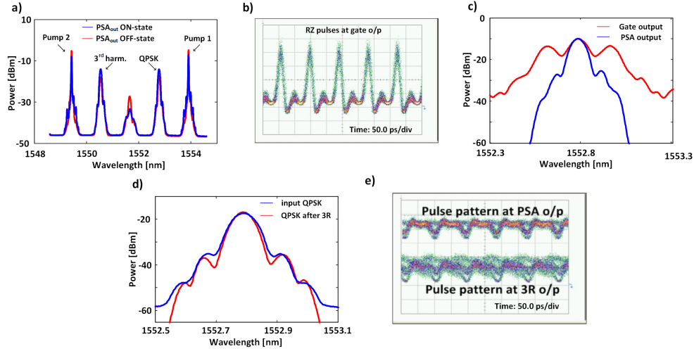
Fig. 5. (a) Optical spectrum at the output of the PSA for both maximum (ON, blue line) and minimum (OFF, red line) phase sensitive gain states (point-A). (b) RZ pulses at the output of the gate (point-B). (c) Optical spectra of the QPSK signal at the outputs of the gate (point-B, broadened) and the PSA (point-A). (d) Optical spectrum of the regenerated and retimed QPSK signal before coherent detection (point-C) overlapped with the input signal for comparison. (e) Pulse patterns at the output of the PSA (point-A) and the 3R (point-C).
