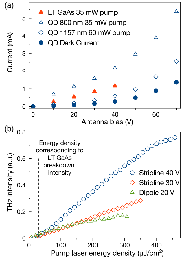
Figure 4 (a) Bias-dependent photocurrent obtained from LT-GaAs and 40 layer QD 50 \mu\text{m} gap stripline antennas, with dark current obtained from QD antenna; (b) THz generation from a 40 layer QD PCA pumped using a fs Ti:Sapphire laser, THz power versus laser pump intensity. Dashed line shows breakdown energy density for LT-GaAs.
