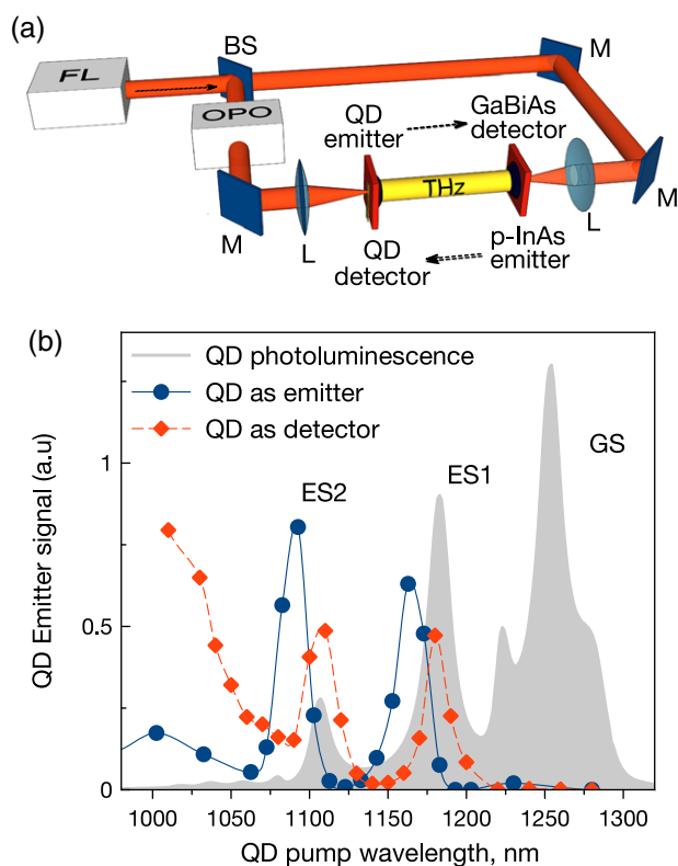
Figure 2 Pump wavelength dependence of QD material in generation and detection regimes and its photoluminescence. (a) Setup layout, for both experiments, arrows depict the difference in THz propagation from corresponding sources to detectors; FL – femtosecond laser, OPO – optical parametric oscillator, BS – beamsplitter, M – mirrors, L – lenses; (b) wavelength dependencies of THz signals emitted by QD sample and registered by GaBiAs detector (blue) and emitted by InAs crystal surface and registered by QD detector (red), GS – ground state, ES1 – first excited state, ES2 – second excited state. Photoluminescence curve is inserted to show wavelengths corresponding to GS and ESs.
