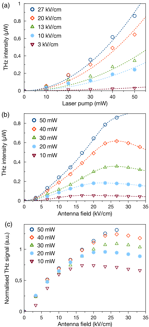
Figure 3 THz generation from a 25 layer QD PCA pumped using a fs Ti:Sapphire laser: (a) THz power versus laser pump power, (b) THz power at different fields applied to antenna. (c) THz signal normalised to the pump power.
