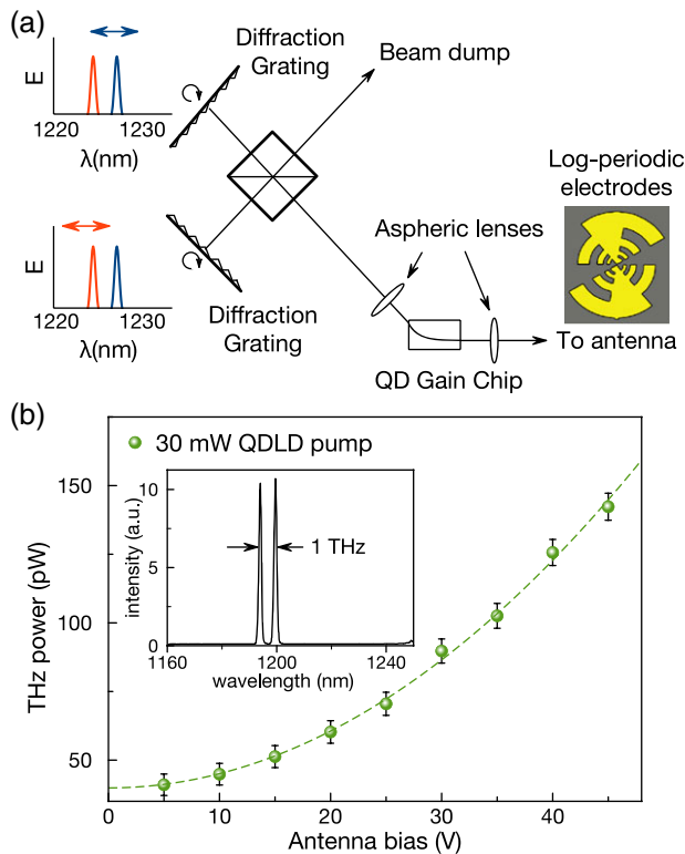
Figure 6 (a) QD LD in the double-Littrow configuration ; (b) CW THz intensity from 5 \mu\text{m} gap log-periodic QD PCA pumped by this laser, measured by low-temperature bolometer. Dashed line shows quadratic fit. Inset: optical spectrum of the QD LD.
