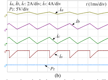
Fig. 23. Experimental results for battery charging in standstill condition. (a) Duty-cycle 0.5. (b) Duty-cycle 0.6.
