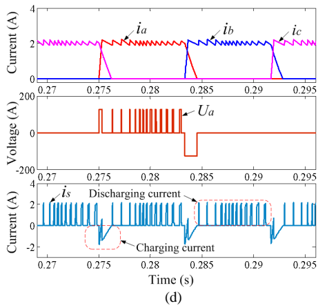
Fig. 13. Simulation results for low-speed operation. (a) Conventional converter without front-end circuit. (b) Powered by the generator. (c) Powered by the battery. (d) Powered by the dual-source.
