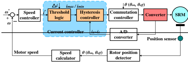
Fig. 3. Block diagram of the speed-controlled SRM system.
