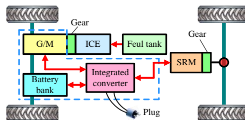
Fig. 1. Diagram of the proposed SRM-based PHEV drivetrain.
