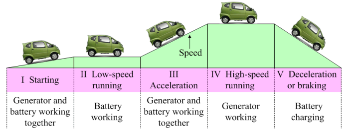
Fig. 11. Cooperation of the generator and the battery working in different speed conditions.
