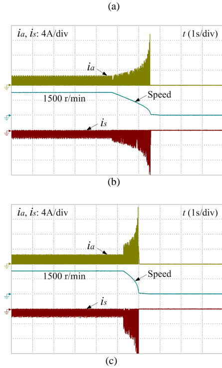
Fig. 22. Experimental results for braking operation. (a) Inertial stopping. (b) Turn-on angle 20^\circ and turn-off angle 30^\circ . (c) Turn-on angle 20^\circ and turn-off angle 40^\circ .
