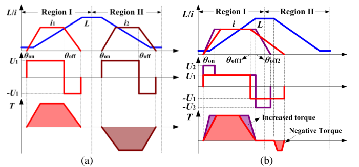
Fig. 2. Relationship of the phase inductance, phase voltage and torque. (a) In motoring and regenerative braking modes. (b) Motoring under different demagnetization voltages.
