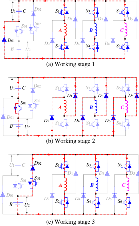
Fig. 9. Working stage of the dual-source energy exchange.
