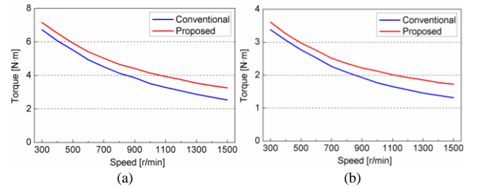
Fig. 24. Torque comparison. (a) Single generator powering mode. (b) Single battery powering mode.
