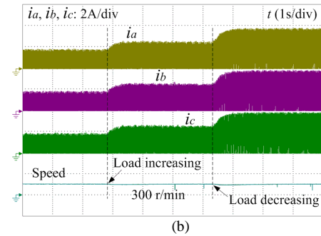
Fig. 21. Experimental results under transient conditions. (a) Speed increasing. (b) Load increasing.
