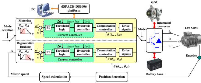
Fig. 17. Experimental diagram of the control system.
