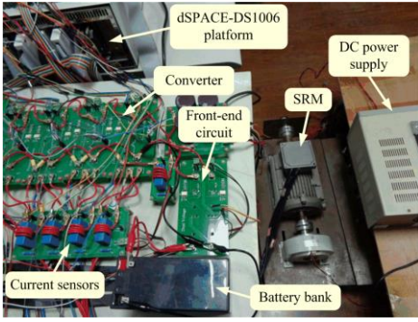
Fig. 16. Experimental setup.
