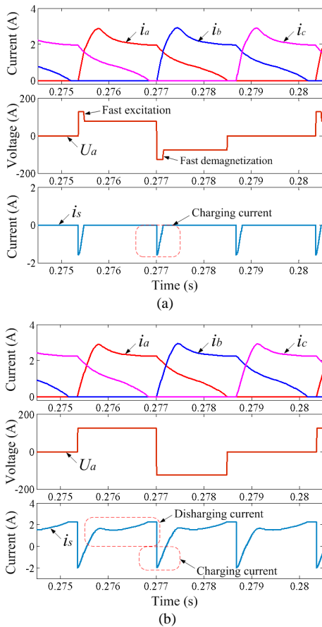
Fig. 14. Simulation results for high-speed operation. (a) Powered by the generator. (b) Powered by the dual-source.
