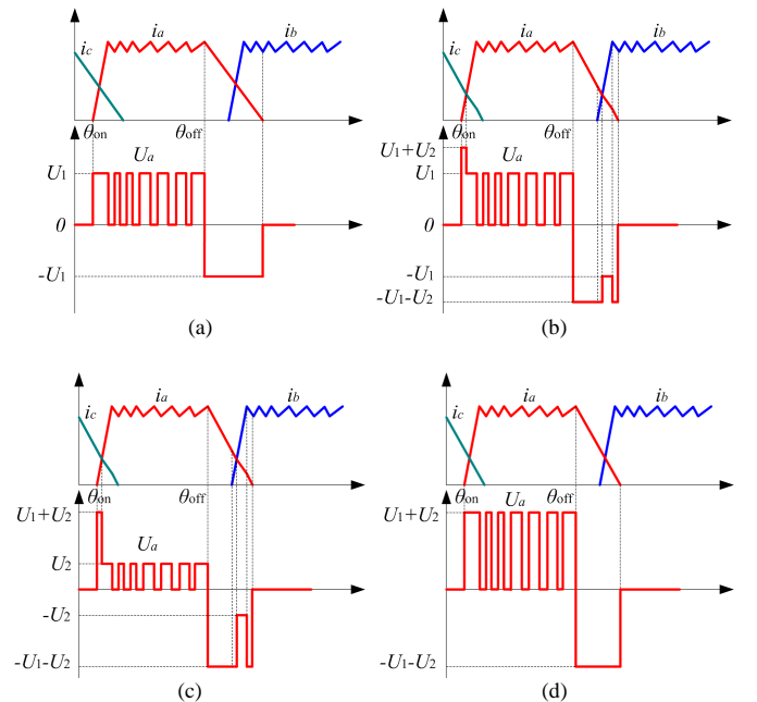
Fig. 8. Phase current and phase voltage. (a) In conventional converter. (b) Powered by the generator in new converter. (c) Powered by the battery in new converter. (d) Powered by the dual-source in new converter.
