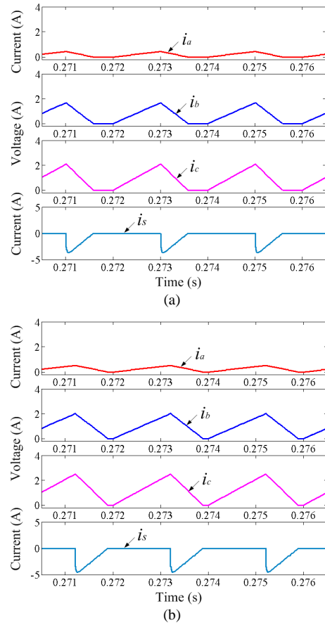
Fig. 15. Simulation results for battery charging in standstill condition. (a) Duty-cycle 0.5. (b) Duty-cycle 0.6.
