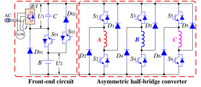
Fig. 4. Proposed integrated converter fed by front-end circuit.
