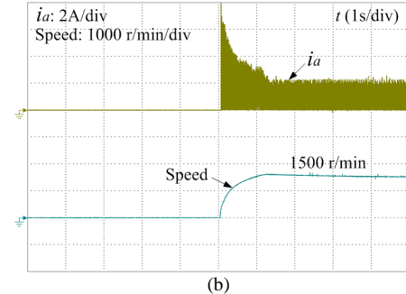
Fig. 20. Experimental results for startup operation. (a) Powered by single generator. (b) Powered by the dual-source.
