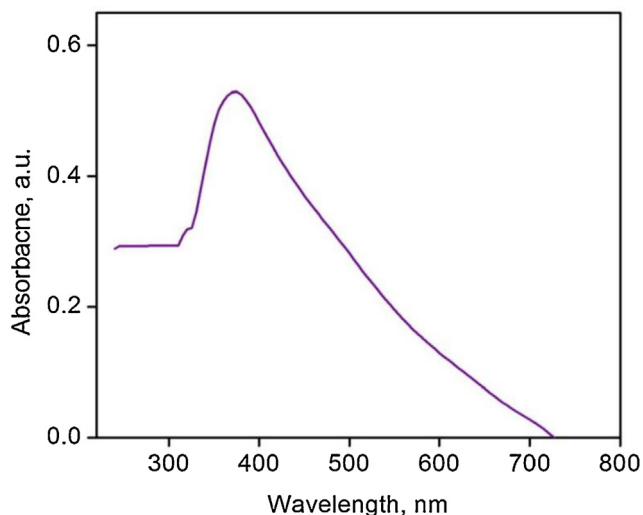
Fig. 3. DRUVS spectrum of CuFe/SBA-15 catalyst.
