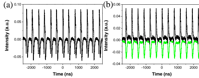
Figure 7 (a) Oscilloscope traces of 2 nd harmonic mode-locking of bright-dark pulse pair, (b) its polarization-resolved oscilloscope traces.
