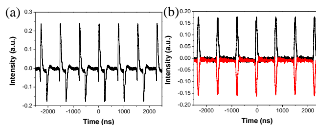
Figure 5 (a) Oscilloscope trace of the bright-dark pulse pair, (b) filtered oscilloscope traces of bright pulse at 1554.8 nm (black curve) and dark pulse at 1560.9 nm (red curve).
