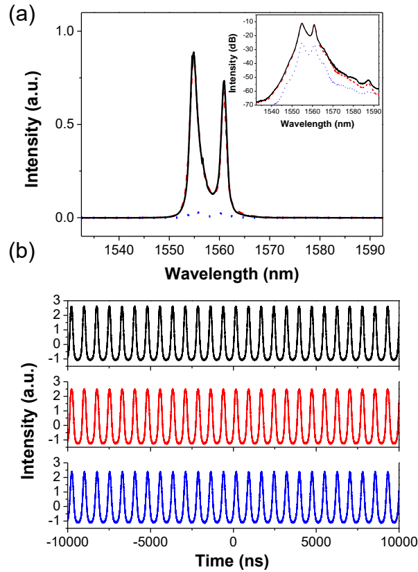
Figure 3 (a) Spectrum of dual-wavelength bright pulse (black solid line) and its polarization-resolved spectra (red dashed and blue dotted lines) on linear scale (inset is on logarithmic scale), (b) corresponding oscilloscope traces (red and blue lines).
