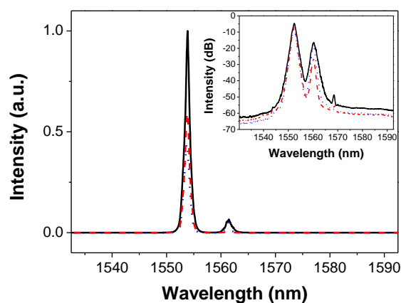
Figure 4 Spectrum of bright-dark pulse pair (black solid line) and its polarization-resolved spectra (red dashed and blue dotted lines) on linear scale (inset is on logarithmic scale).
