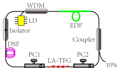
Figure 1 Schematic of mode-locked fiber laser with an LA-TFG.
