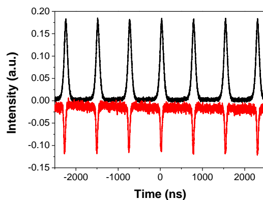
Figure 6 Polarization-resolved oscilloscope traces of the bright-dark pulse pair at two orthogonal axes.
