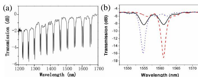
Figure 2 Measured transmission of the LA-TFG (a) from 1200 nm to 1700 nm range and (b) from 1548 nm to 1572 nm range under different polarization excitation.
