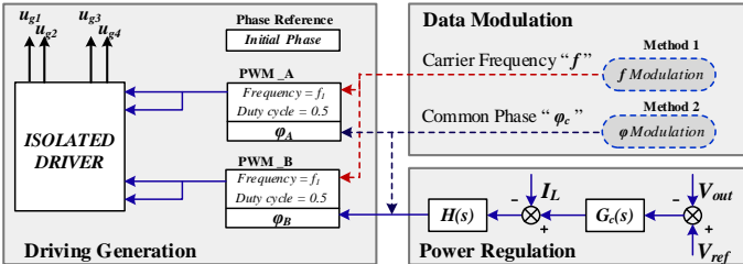
Fig.4 Control scheme of phase shift full bridge converter.
