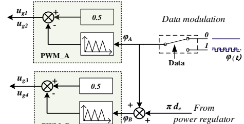
Fig.5 Principle of the phase modulation.
