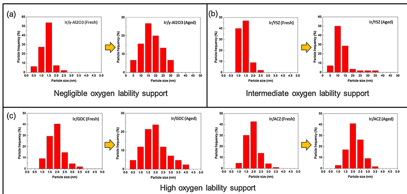
Fig. 5. TEM size distribution profiles for fresh and aged samples; (a) Ir/ \gamma -Al 2 O 3 , (b) Ir/YSZ and (c) Ir/GDC and Ir/ACZ.
