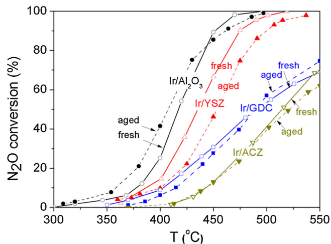
Fig. 8. N 2 O conversion performance of the catalysts as a function of temperature (light-off diagram). Conditions: w cat = 50 mg; Feed composition: 1000 ppm N 2 O/He, Ft = 150 cm 3 min -1 ; Weight hourly space velocity, WHSV = 180,000 cm 3 g -1 h -1 .
