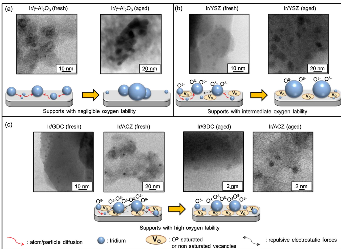
Fig. 4. TEM images of fresh and aged samples; (a) Ir/ \gamma -Al 2 O 3 , (b) Ir/YSZ and (c) Ir/GDC and Ir/ACZ. Also shown are possible models for catalyst particle nanoparticle stabilization on supports with high oxygen ion lability and storage capacity.
