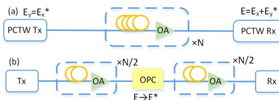
Fig. 1. Illustration of PCTW (a) and mid-link OPC (b) for fiber nonlinearity compensation, OA – optical amplifier, N – number of span.
